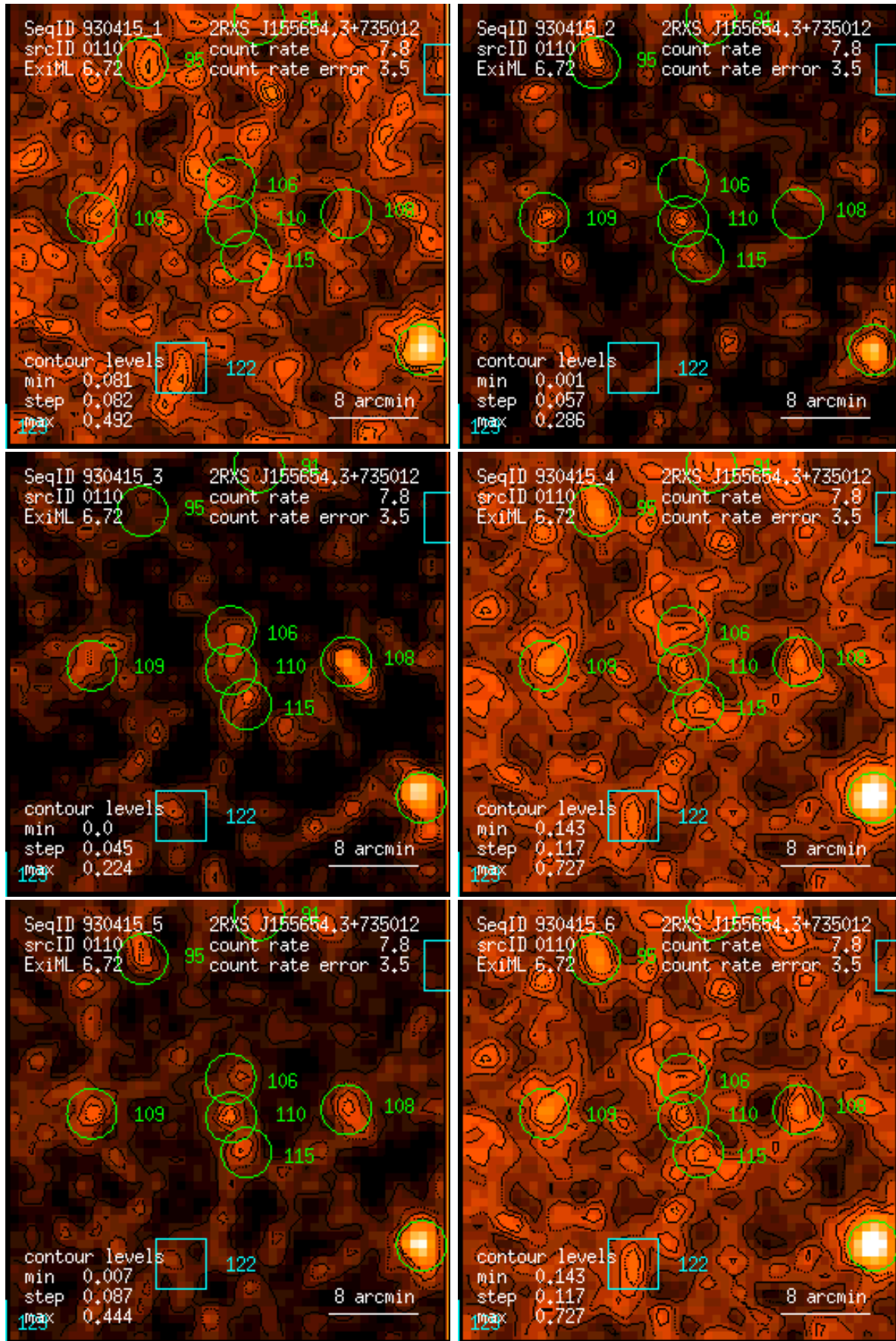
Figure 110: RASS 930415: detection 0110: band rate images, Gaussian filter: (1) PSPC channels 11 – 41, (2) 52 – 90, (3) 91 – 201, (4) 11 – 235, (5) 52 – 201, (6) 11 – 201. Broad band rates in counts/ks. Band rate contour levels in counts/ks/arcmin 2 .
