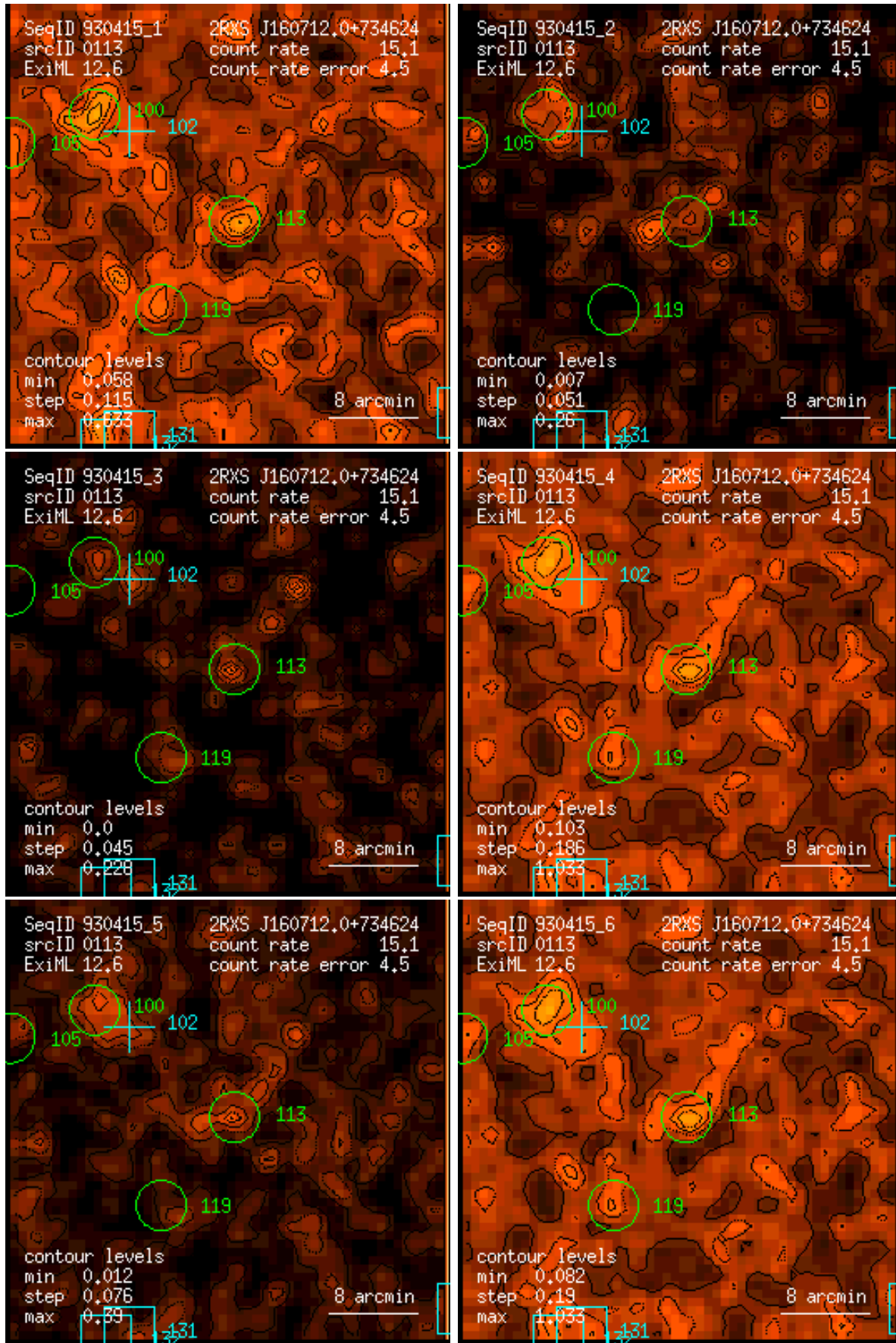
Figure 113: RASS 930415: detection 0113: band rate images, Gaussian filter: (1) PSPC channels 11 – 41, (2) 52 – 90, (3) 91 – 201, (4) 11 – 235, (5) 52 – 201, (6) 11 – 201. Broad band rates in counts/ks. Band rate contour levels in counts/ks/arcmin 2 .
