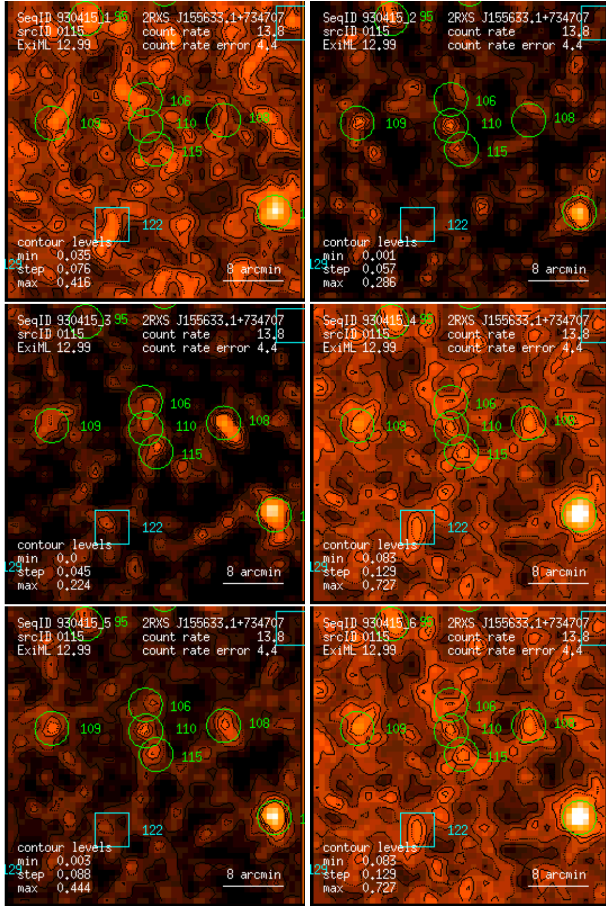
Figure 115: RASS 930415: detection 0115: band rate images, Gaussian filter: (1) PSPC channels 11 – 41, (2) 52 – 90, (3) 91 – 201, (4) 11 – 235, (5) 52 – 201, (6) 11 – 201. Broad band rates in counts/ks. Band rate contour levels in counts/ks/arcmin 2 .
