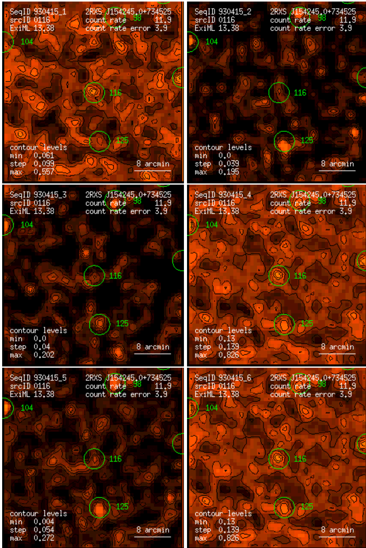
Figure 116: RASS 930415: detection 0116: band rate images, Gaussian filter: (1) PSPC channels 11 – 41, (2) 52 – 90, (3) 91 – 201, (4) 11 – 235, (5) 52 – 201, (6) 11 – 201. Broad band rates in counts/ks. Band rate contour levels in counts/ks/arcmin 2 .
