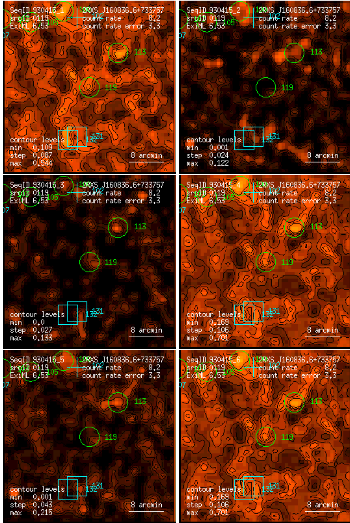
Figure 119: RASS 930415: detection 0119: band rate images, Gaussian filter: (1) PSPC channels 11 – 41, (2) 52 – 90, (3) 91 – 201, (4) 11 – 235, (5) 52 – 201, (6) 11 – 201. Broad band rates in counts/ks. Band rate contour levels in counts/ks/arcmin 2 .
