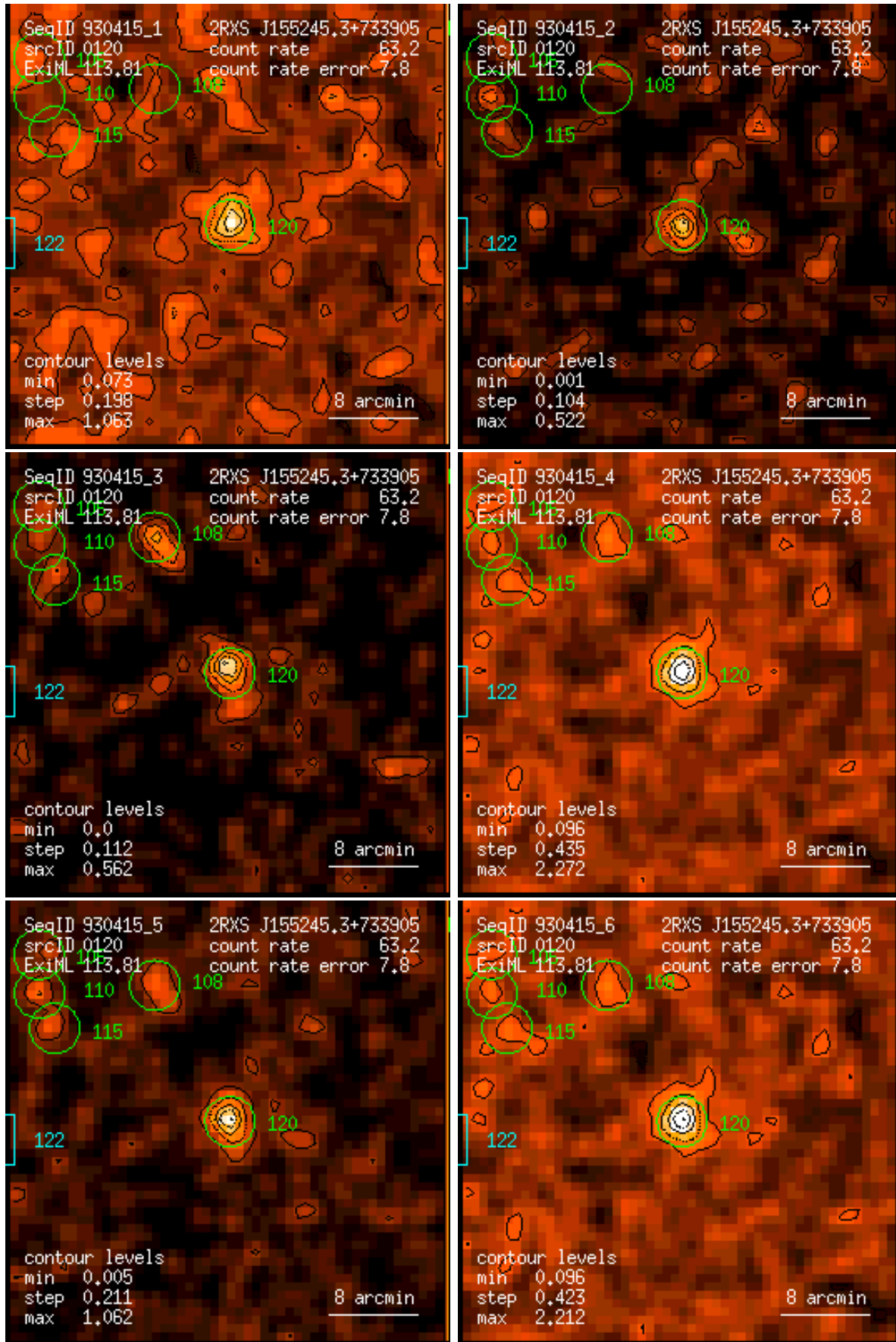
Figure 120: RASS 930415: detection 0120: band rate images, Gaussian filter: (1) PSPC channels 11 – 41, (2) 52 – 90, (3) 91 – 201, (4) 11 – 235, (5) 52 – 201, (6) 11 – 201. Broad band rates in counts/ks. Band rate contour levels in counts/ks/arcmin 2 .
