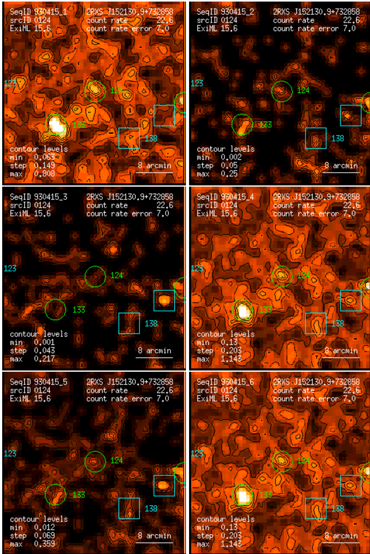
Figure 124: RASS 930415: detection 0124: band rate images, Gaussian filter: (1) PSPC channels 11 – 41, (2) 52 – 90, (3) 91 – 201, (4) 11 – 235, (5) 52 – 201, (6) 11 – 201. Broad band rates in counts/ks. Band rate contour levels in counts/ks/arcmin 2 .
