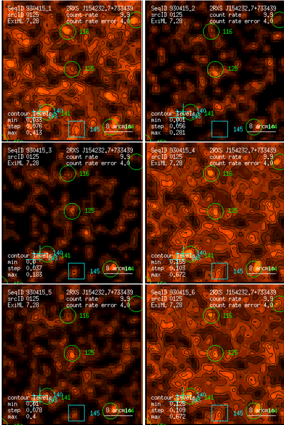
Figure 125: RASS 930415: detection 0125: band rate images, Gaussian filter: (1) PSPC channels 11 – 41, (2) 52 – 90, (3) 91 – 201, (4) 11 – 235, (5) 52 – 201, (6) 11 – 201. Broad band rates in counts/ks. Band rate contour levels in counts/ks/arcmin 2 .
