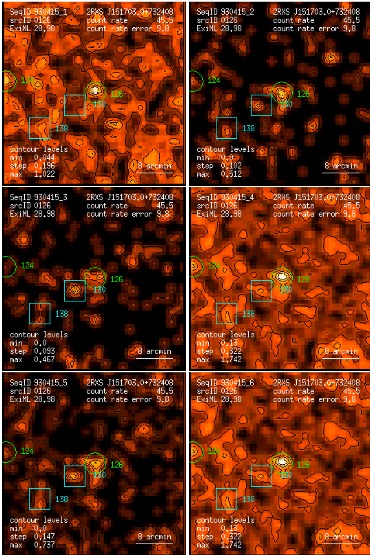
Figure 126: RASS 930415: detection 0126: band rate images, Gaussian filter: (1) PSPC channels 11 – 41, (2) 52 – 90, (3) 91 – 201, (4) 11 – 235, (5) 52 – 201, (6) 11 – 201. Broad band rates in counts/ks. Band rate contour levels in counts/ks/arcmin 2 .
