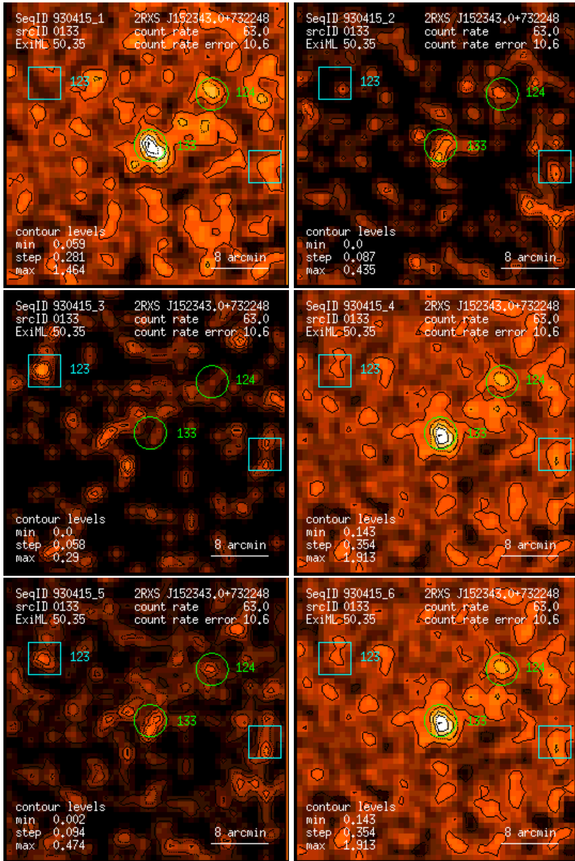
Figure 133: RASS 930415: detection 0133: band rate images, Gaussian filter: (1) PSPC channels 11 – 41, (2) 52 – 90, (3) 91 – 201, (4) 11 – 235, (5) 52 – 201, (6) 11 – 201. Broad band rates in counts/ks. Band rate contour levels in counts/ks/arcmin 2 .
