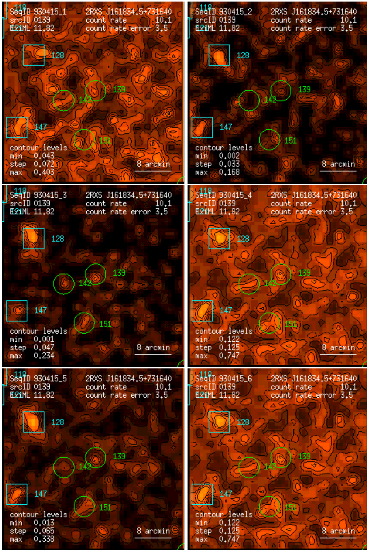
Figure 139: RASS 930415: detection 0139: band rate images, Gaussian filter: (1) PSPC channels 11 – 41, (2) 52 – 90, (3) 91 – 201, (4) 11 – 235, (5) 52 – 201, (6) 11 – 201. Broad band rates in counts/ks. Band rate contour levels in counts/ks/arcmin 2 .
