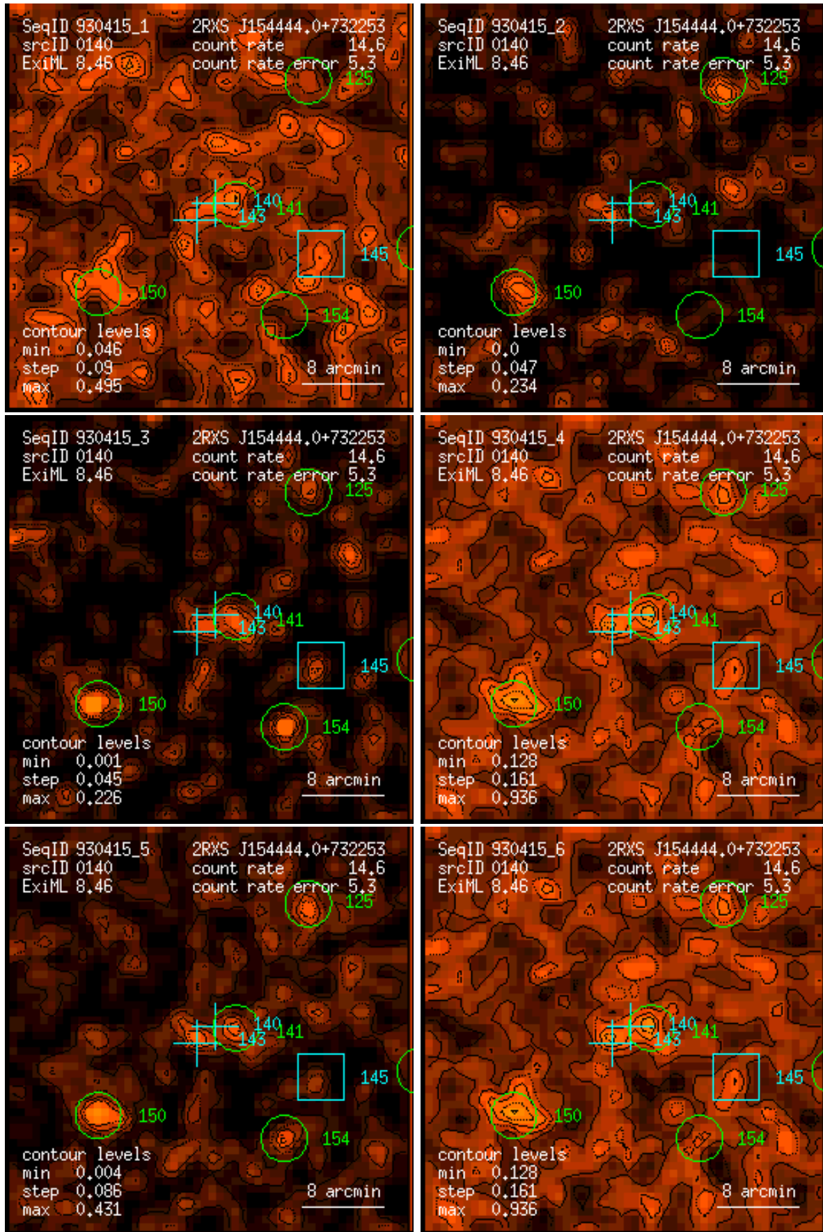
Figure 140: RASS 930415: detection 0140: band rate images, Gaussian filter: (1) PSPC channels 11 – 41, (2) 52 – 90, (3) 91 – 201, (4) 11 – 235, (5) 52 – 201, (6) 11 – 201. Broad band rates in counts/ks. Band rate contour levels in counts/ks/arcmin 2 .
