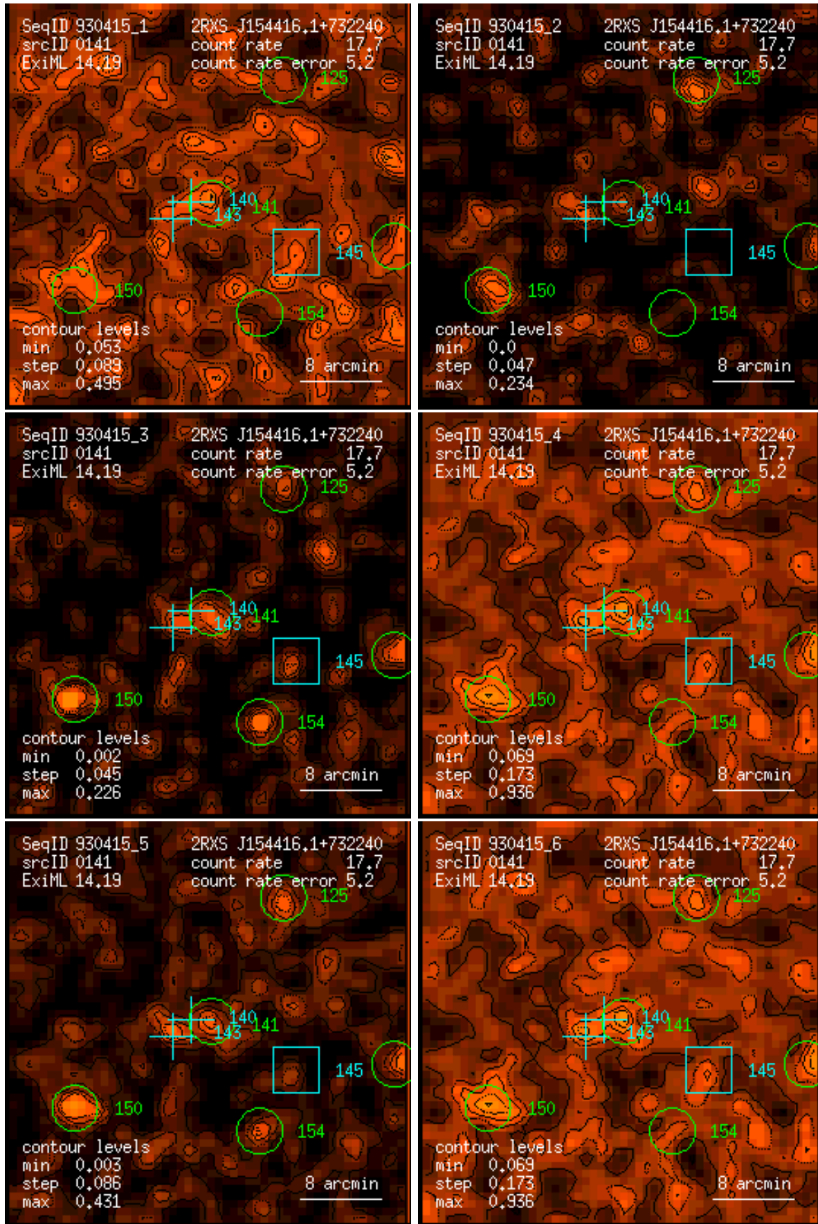
Figure 141: RASS 930415: detection 0141: band rate images, Gaussian filter: (1) PSPC channels 11 – 41, (2) 52 – 90, (3) 91 – 201, (4) 11 – 235, (5) 52 – 201, (6) 11 – 201. Broad band rates in counts/ks. Band rate contour levels in counts/ks/arcmin 2 .
