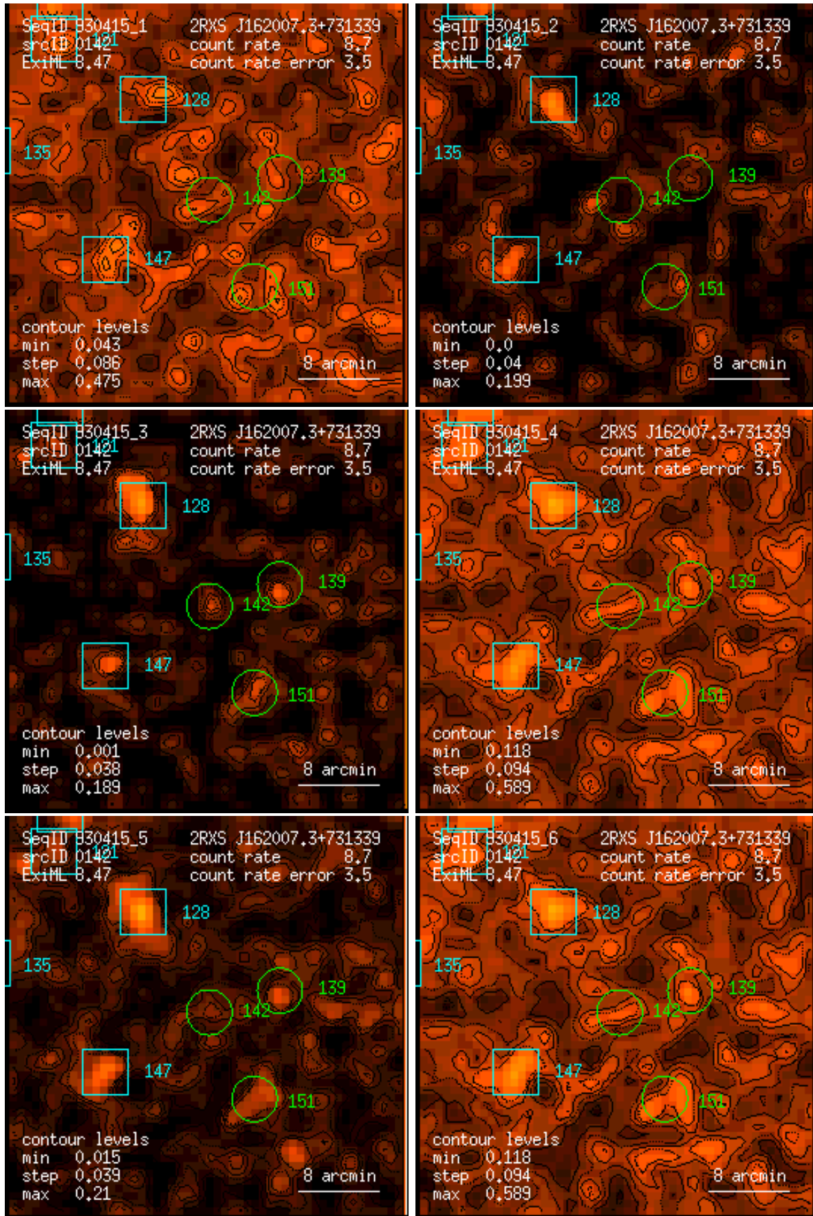
Figure 142: RASS 930415: detection 0142: band rate images, Gaussian filter: (1) PSPC channels 11 – 41, (2) 52 – 90, (3) 91 – 201, (4) 11 – 235, (5) 52 – 201, (6) 11 – 201. Broad band rates in counts/ks. Band rate contour levels in counts/ks/arcmin 2 .
