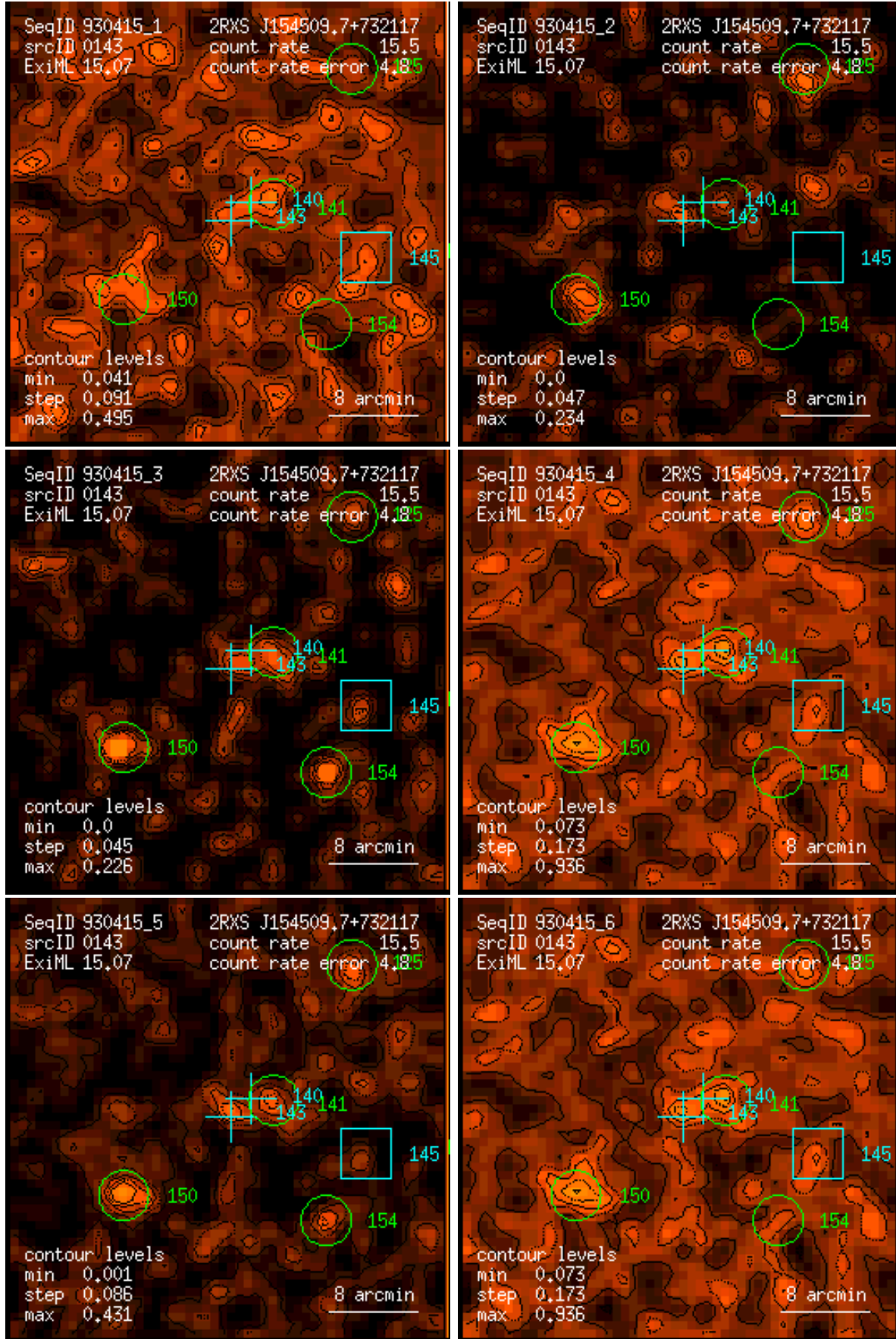
Figure 143: RASS 930415: detection 0143: band rate images, Gaussian filter: (1) PSPC channels 11 – 41, (2) 52 – 90, (3) 91 – 201, (4) 11 – 235, (5) 52 – 201, (6) 11 – 201. Broad band rates in counts/ks. Band rate contour levels in counts/ks/arcmin 2 .
