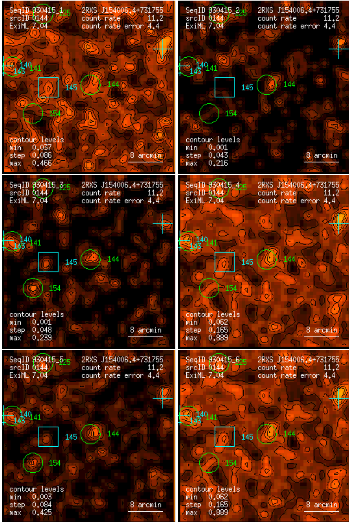
Figure 144: RASS 930415: detection 0144: band rate images, Gaussian filter: (1) PSPC channels 11 – 41, (2) 52 – 90, (3) 91 – 201, (4) 11 – 235, (5) 52 – 201, (6) 11 – 201. Broad band rates in counts/ks. Band rate contour levels in counts/ks/arcmin 2 .
