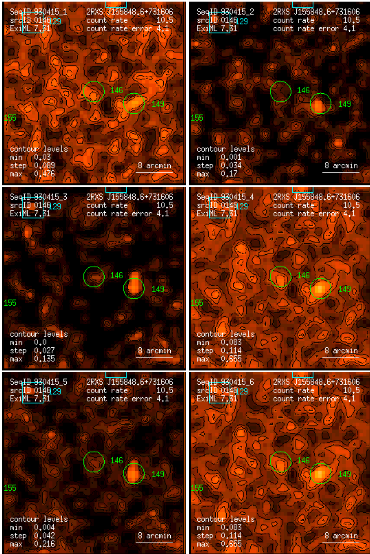
Figure 146: RASS 930415: detection 0146: band rate images, Gaussian filter: (1) PSPC channels 11 – 41, (2) 52 – 90, (3) 91 – 201, (4) 11 – 235, (5) 52 – 201, (6) 11 – 201. Broad band rates in counts/ks. Band rate contour levels in counts/ks/arcmin 2 .
