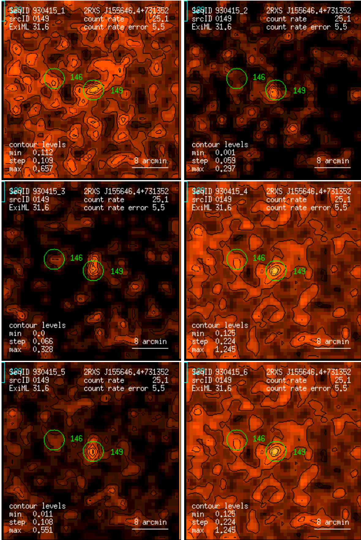
Figure 149: RASS 930415: detection 0149: band rate images, Gaussian filter: (1) PSPC channels 11 – 41, (2) 52 – 90, (3) 91 – 201, (4) 11 – 235, (5) 52 – 201, (6) 11 – 201. Broad band rates in counts/ks. Band rate contour levels in counts/ks/arcmin 2 .
