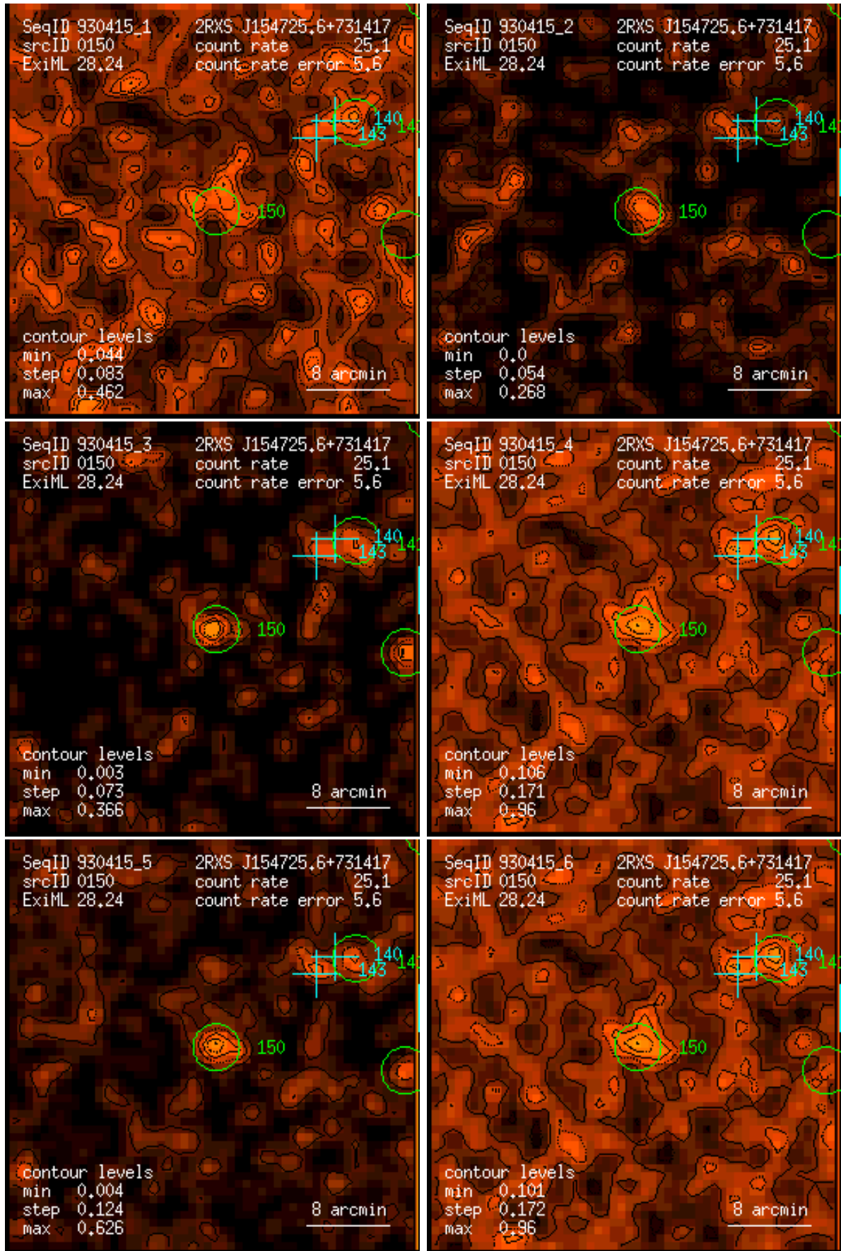
Figure 150: RASS 930415: detection 0150: band rate images, Gaussian filter: (1) PSPC channels 11 – 41, (2) 52 – 90, (3) 91 – 201, (4) 11 – 235, (5) 52 – 201, (6) 11 – 201. Broad band rates in counts/ks. Band rate contour levels in counts/ks/arcmin 2 .
