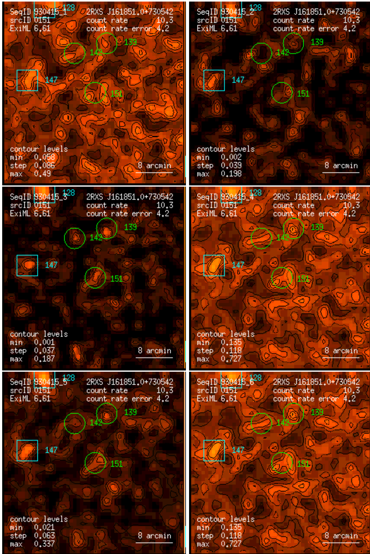
Figure 151: RASS 930415: detection 0151: band rate images, Gaussian filter: (1) PSPC channels 11 – 41, (2) 52 – 90, (3) 91 – 201, (4) 11 – 235, (5) 52 – 201, (6) 11 – 201. Broad band rates in counts/ks. Band rate contour levels in counts/ks/arcmin 2 .
