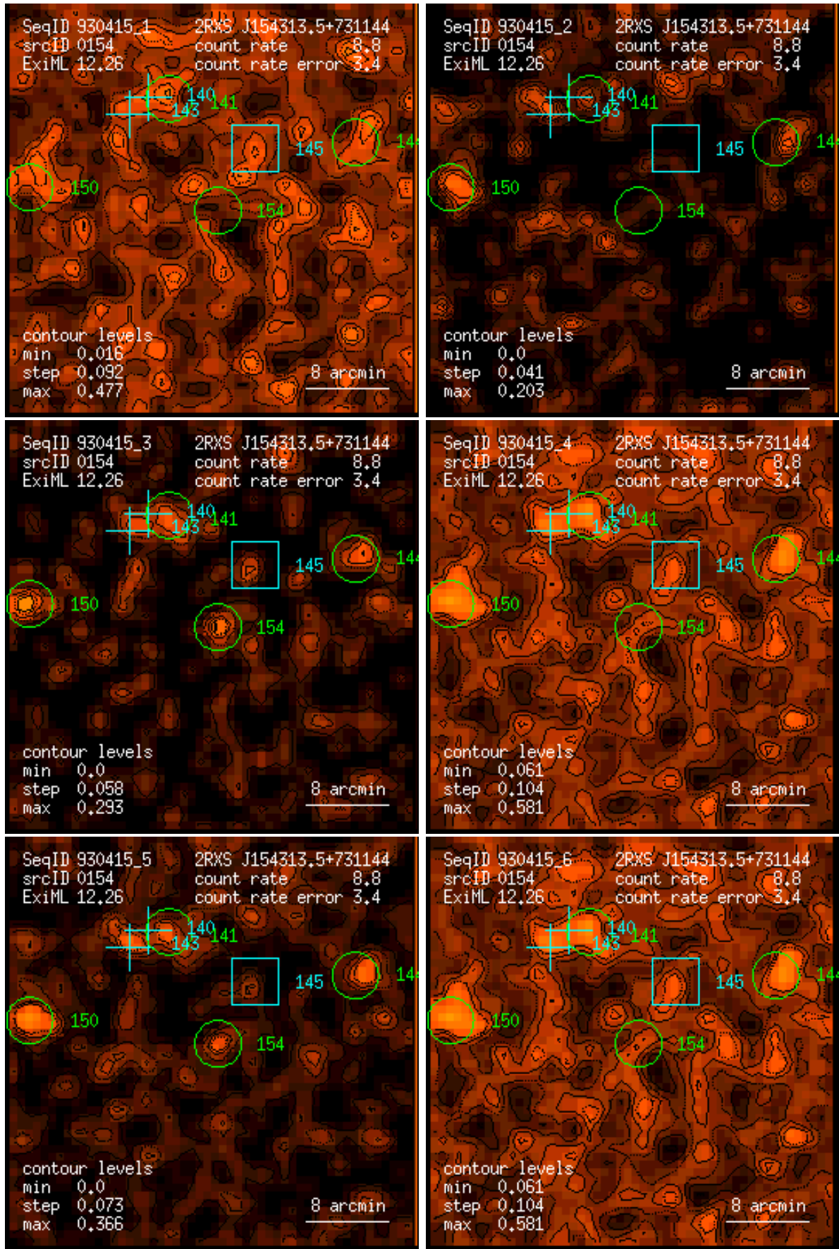
Figure 154: RASS 930415: detection 0154: band rate images, Gaussian filter: (1) PSPC channels 11 – 41, (2) 52 – 90, (3) 91 – 201, (4) 11 – 235, (5) 52 – 201, (6) 11 – 201. Broad band rates in counts/ks. Band rate contour levels in counts/ks/arcmin 2 .
