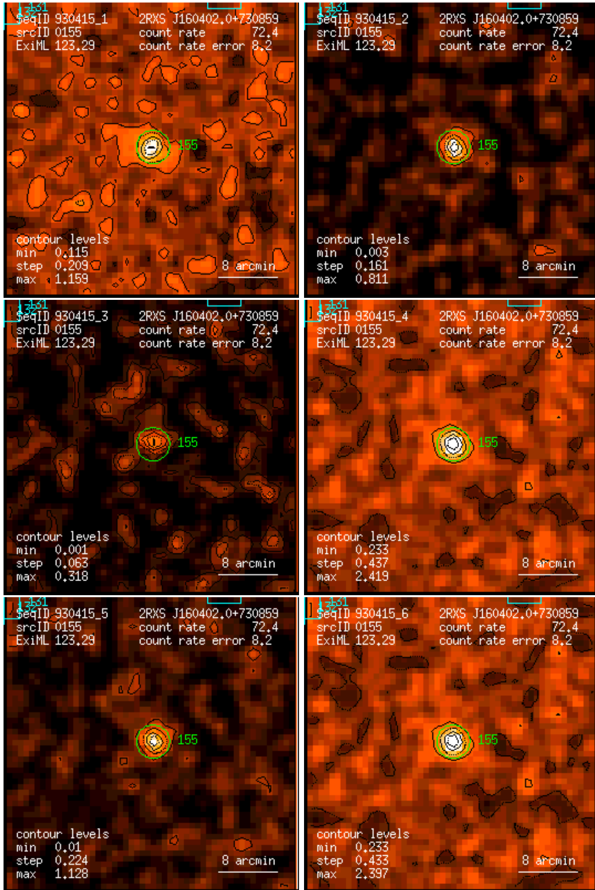
Figure 155: RASS 930415: detection 0155: band rate images, Gaussian filter: (1) PSPC channels 11 – 41, (2) 52 – 90, (3) 91 – 201, (4) 11 – 235, (5) 52 – 201, (6) 11 – 201. Broad band rates in counts/ks. Band rate contour levels in counts/ks/arcmin 2 .
