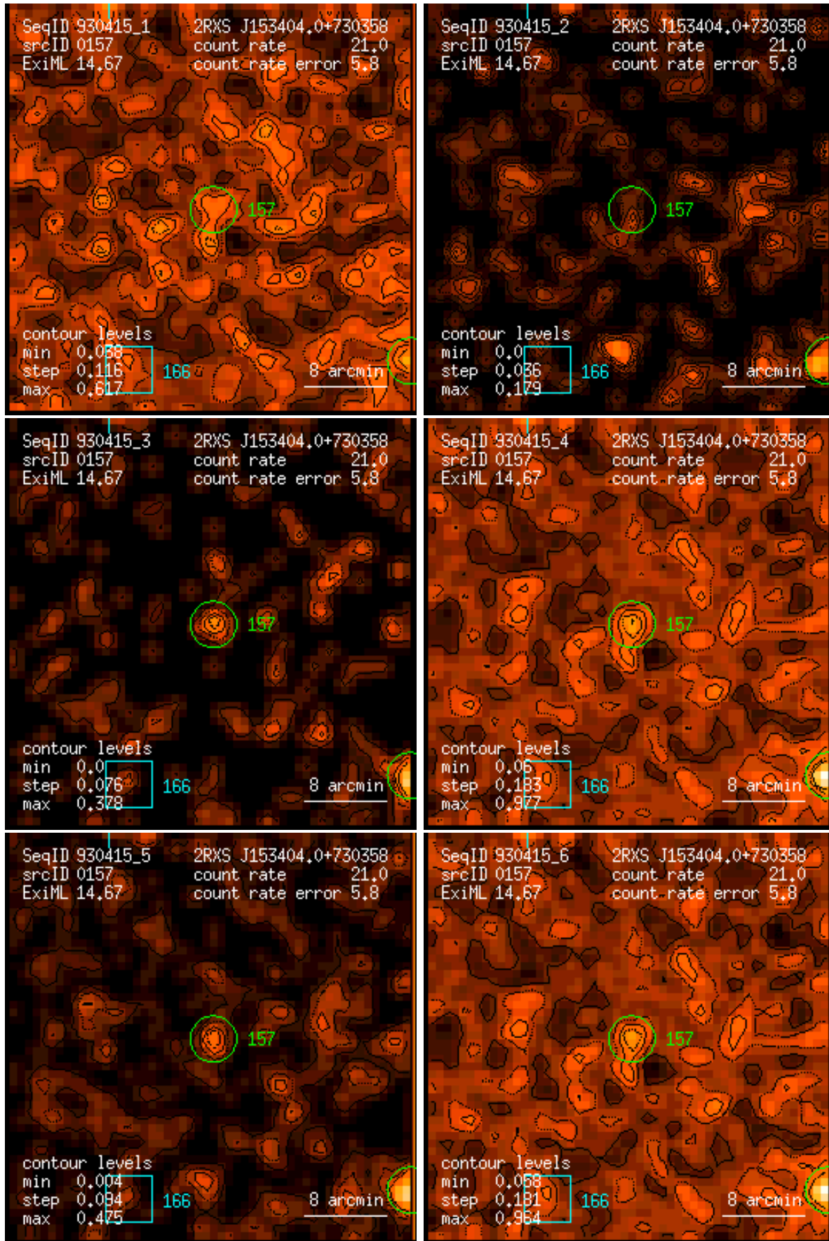
Figure 157: RASS 930415: detection 0157: band rate images, Gaussian filter: (1) PSPC channels 11 – 41, (2) 52 – 90, (3) 91 – 201, (4) 11 – 235, (5) 52 – 201, (6) 11 – 201. Broad band rates in counts/ks. Band rate contour levels in counts/ks/arcmin 2 .
