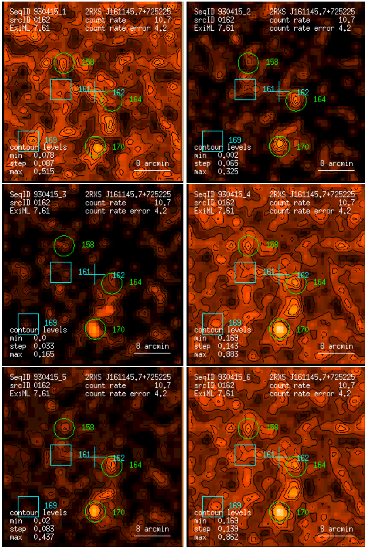
Figure 162: RASS 930415: detection 0162: band rate images, Gaussian filter: (1) PSPC channels 11 – 41, (2) 52 – 90, (3) 91 – 201, (4) 11 – 235, (5) 52 – 201, (6) 11 – 201. Broad band rates in counts/ks. Band rate contour levels in counts/ks/arcmin 2 .
