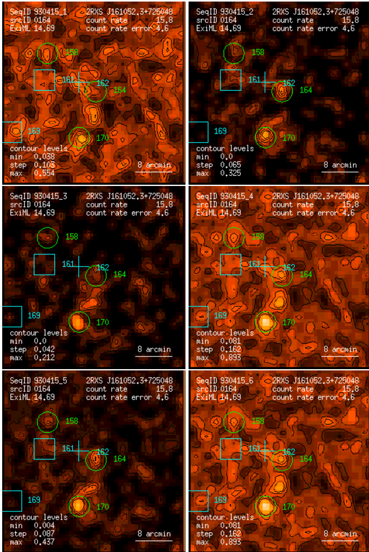
Figure 164: RASS 930415: detection 0164: band rate images, Gaussian filter: (1) PSPC channels 11 – 41, (2) 52 – 90, (3) 91 – 201, (4) 11 – 235, (5) 52 – 201, (6) 11 – 201. Broad band rates in counts/ks. Band rate contour levels in counts/ks/arcmin 2 .
