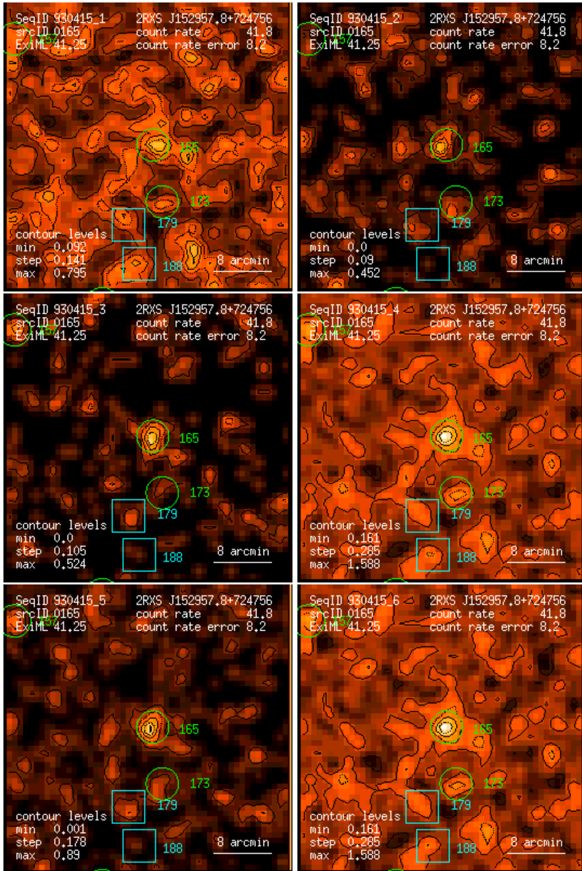
Figure 165: RASS 930415: detection 0165: band rate images, Gaussian filter: (1) PSPC channels 11 – 41, (2) 52 – 90, (3) 91 – 201, (4) 11 – 235, (5) 52 – 201, (6) 11 – 201. Broad band rates in counts/ks. Band rate contour levels in counts/ks/arcmin 2 .
