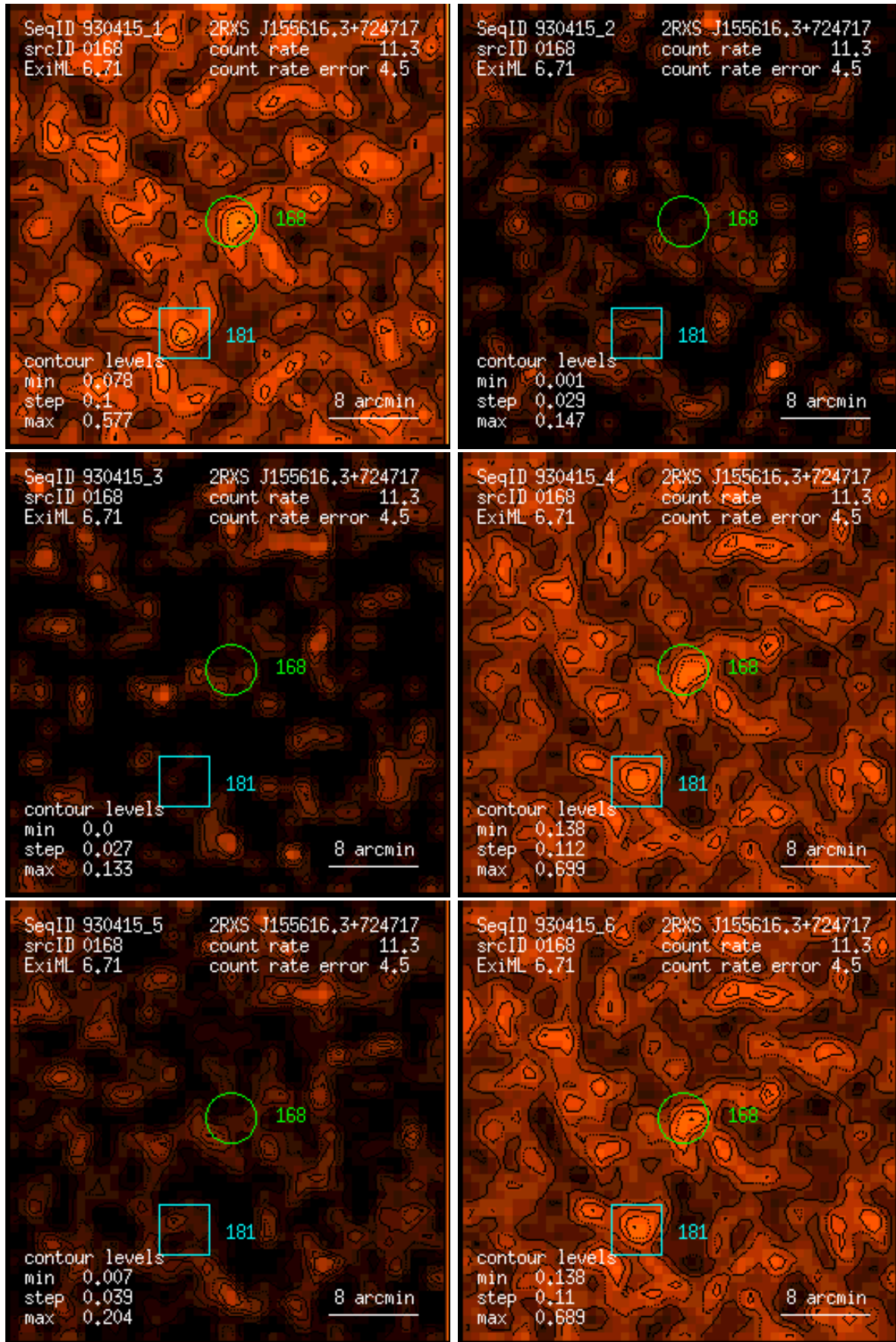
Figure 168: RASS 930415: detection 0168: band rate images, Gaussian filter: (1) PSPC channels 11 – 41, (2) 52 – 90, (3) 91 – 201, (4) 11 – 235, (5) 52 – 201, (6) 11 – 201. Broad band rates in counts/ks. Band rate contour levels in counts/ks/arcmin 2 .
