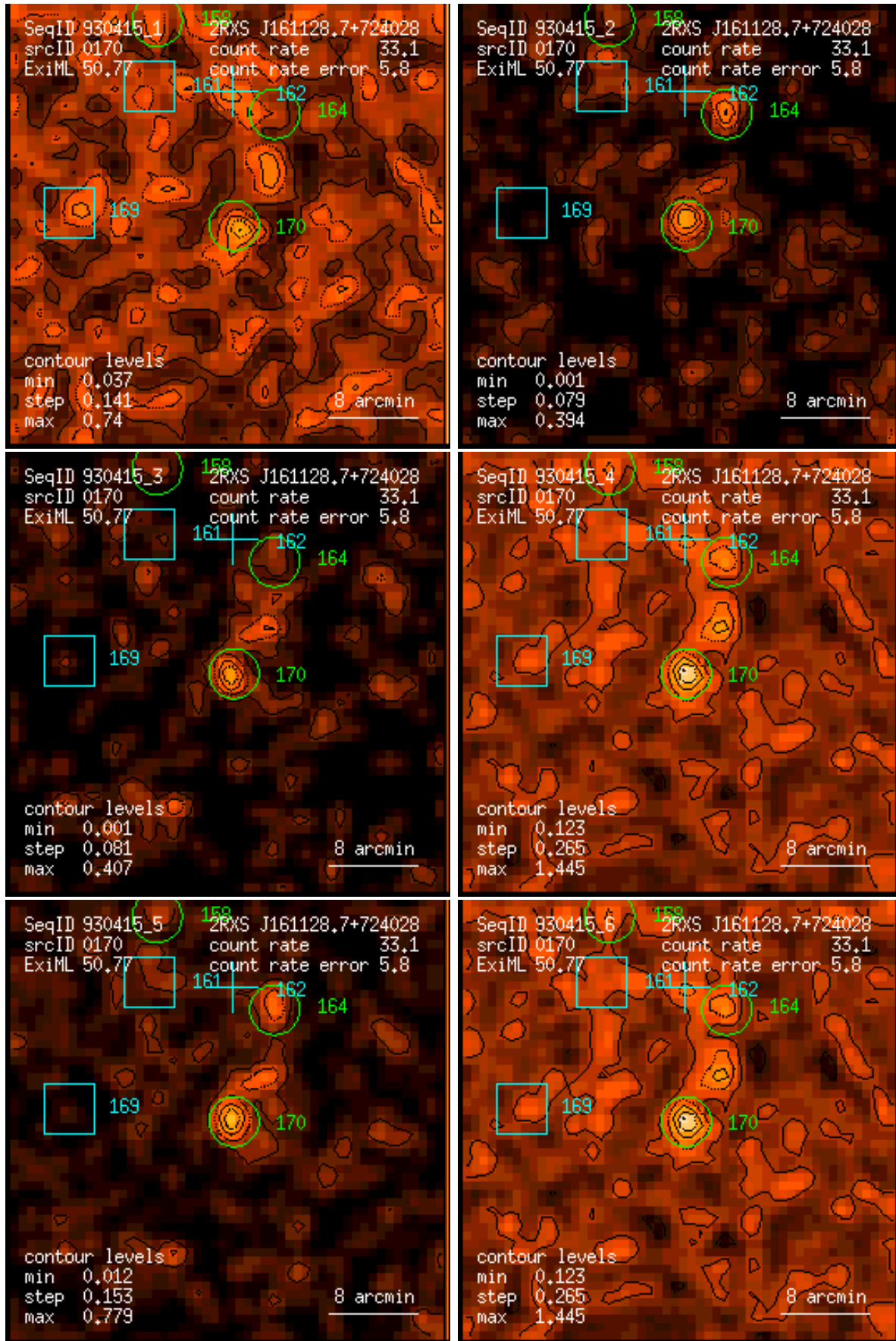
Figure 170: RASS 930415: detection 0170: band rate images, Gaussian filter: (1) PSPC channels 11 – 41, (2) 52 – 90, (3) 91 – 201, (4) 11 – 235, (5) 52 – 201, (6) 11 – 201. Broad band rates in counts/ks. Band rate contour levels in counts/ks/arcmin 2 .
