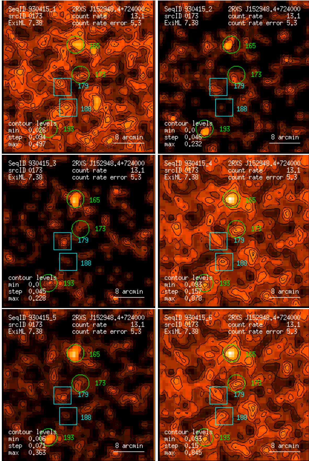
Figure 173: RASS 930415: detection 0173: band rate images, Gaussian filter: (1) PSPC channels 11 – 41, (2) 52 – 90, (3) 91 – 201, (4) 11 – 235, (5) 52 – 201, (6) 11 – 201. Broad band rates in counts/ks. Band rate contour levels in counts/ks/arcmin 2 .
