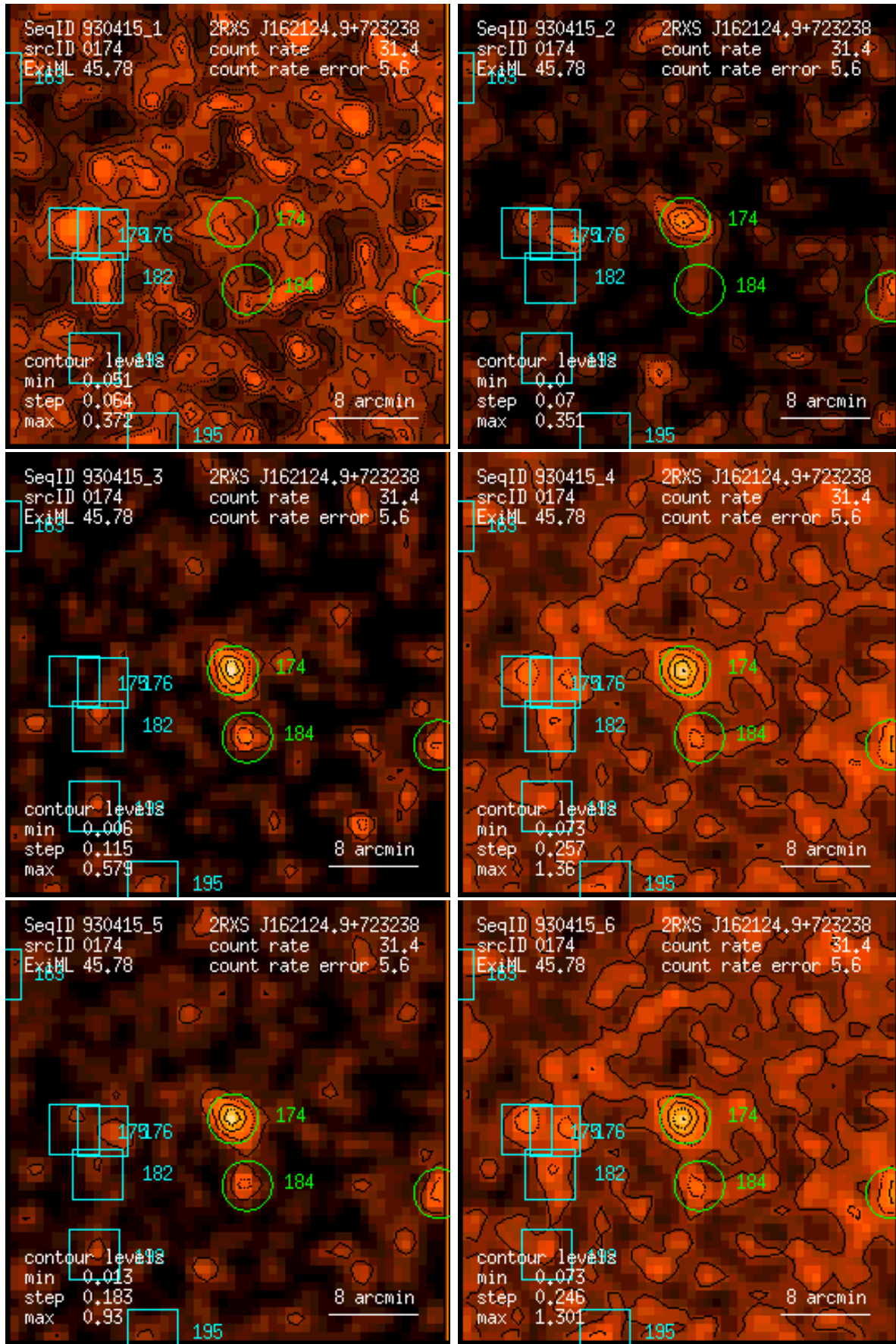
Figure 174: RASS 930415: detection 0174: band rate images, Gaussian filter: (1) PSPC channels 11 – 41, (2) 52 – 90, (3) 91 – 201, (4) 11 – 235, (5) 52 – 201, (6) 11 – 201. Broad band rates in counts/ks. Band rate contour levels in counts/ks/arcmin 2 .
