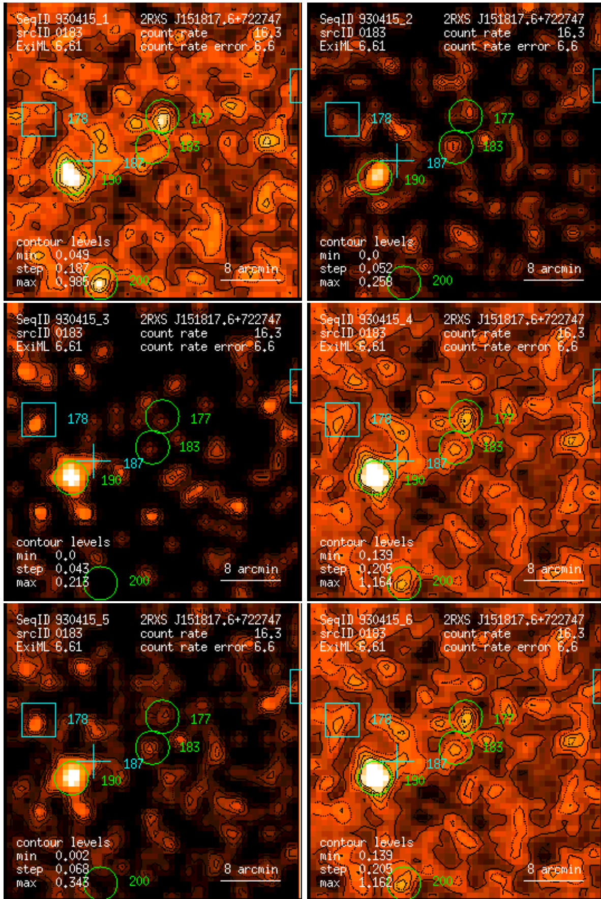
Figure 183: RASS 930415: detection 0183: band rate images, Gaussian filter: (1) PSPC channels 11 – 41, (2) 52 – 90, (3) 91 – 201, (4) 11 – 235, (5) 52 – 201, (6) 11 – 201. Broad band rates in counts/ks. Band rate contour levels in counts/ks/arcmin 2 .
