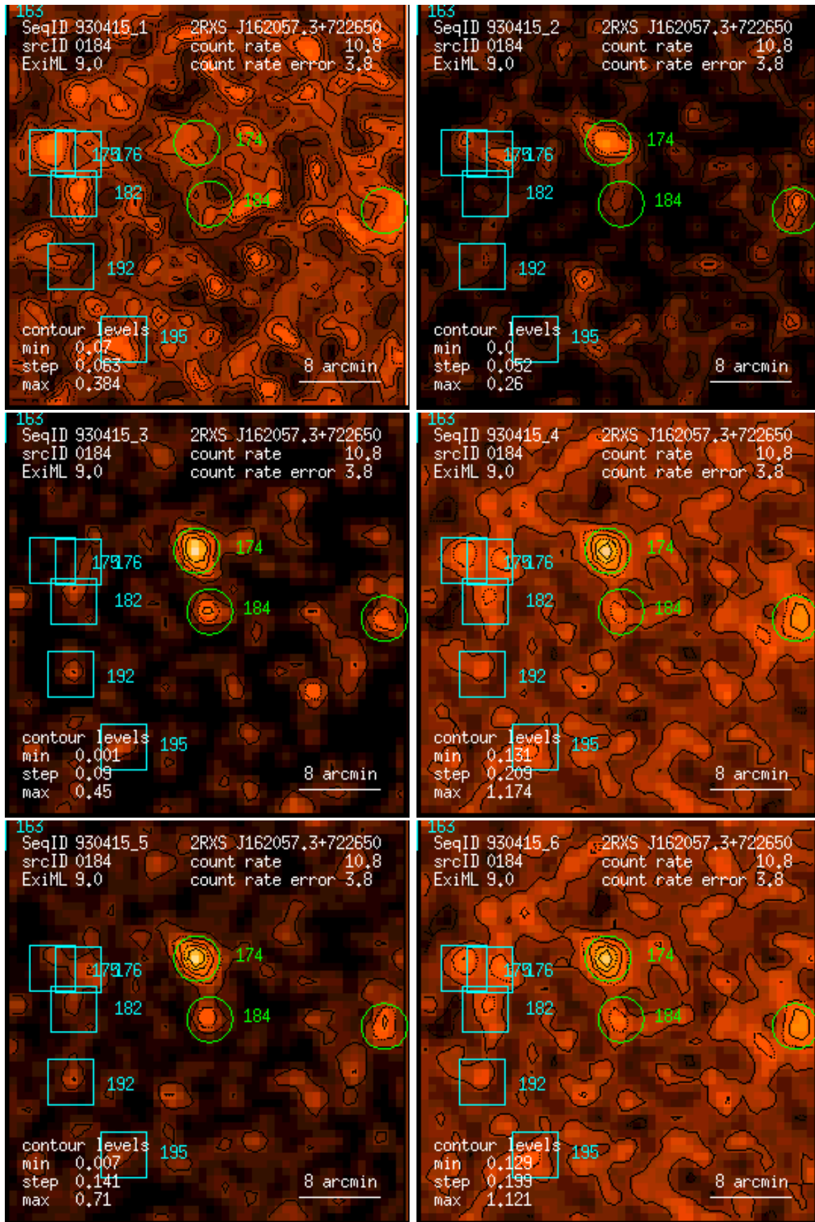
Figure 184: RASS 930415: detection 0184: band rate images, Gaussian filter: (1) PSPC channels 11 – 41, (2) 52 – 90, (3) 91 – 201, (4) 11 – 235, (5) 52 – 201, (6) 11 – 201. Broad band rates in counts/ks. Band rate contour levels in counts/ks/arcmin 2 .
