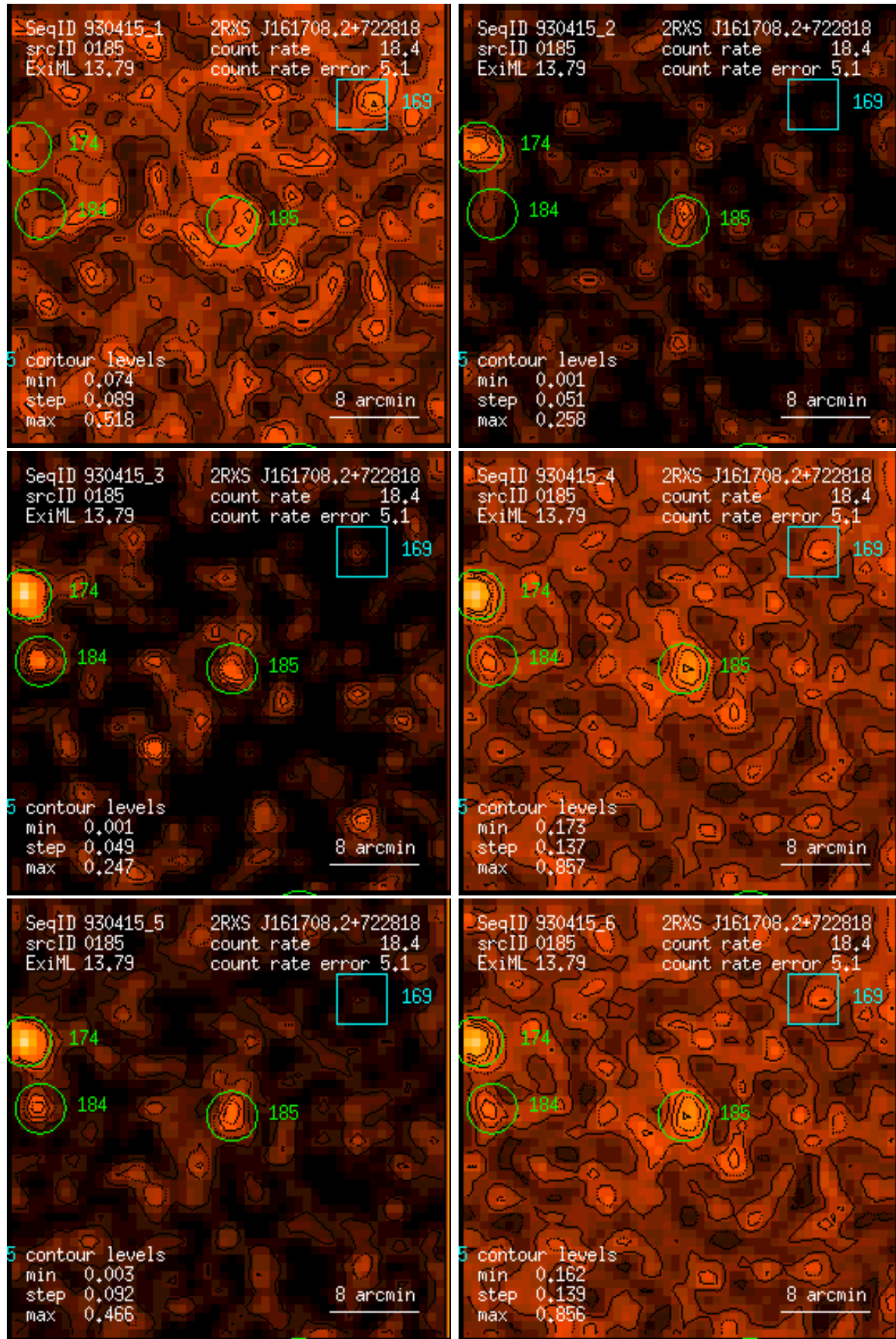
Figure 185: RASS 930415: detection 0185: band rate images, Gaussian filter: (1) PSPC channels 11 – 41, (2) 52 – 90, (3) 91 – 201, (4) 11 – 235, (5) 52 – 201, (6) 11 – 201. Broad band rates in counts/ks. Band rate contour levels in counts/ks/arcmin 2 .
