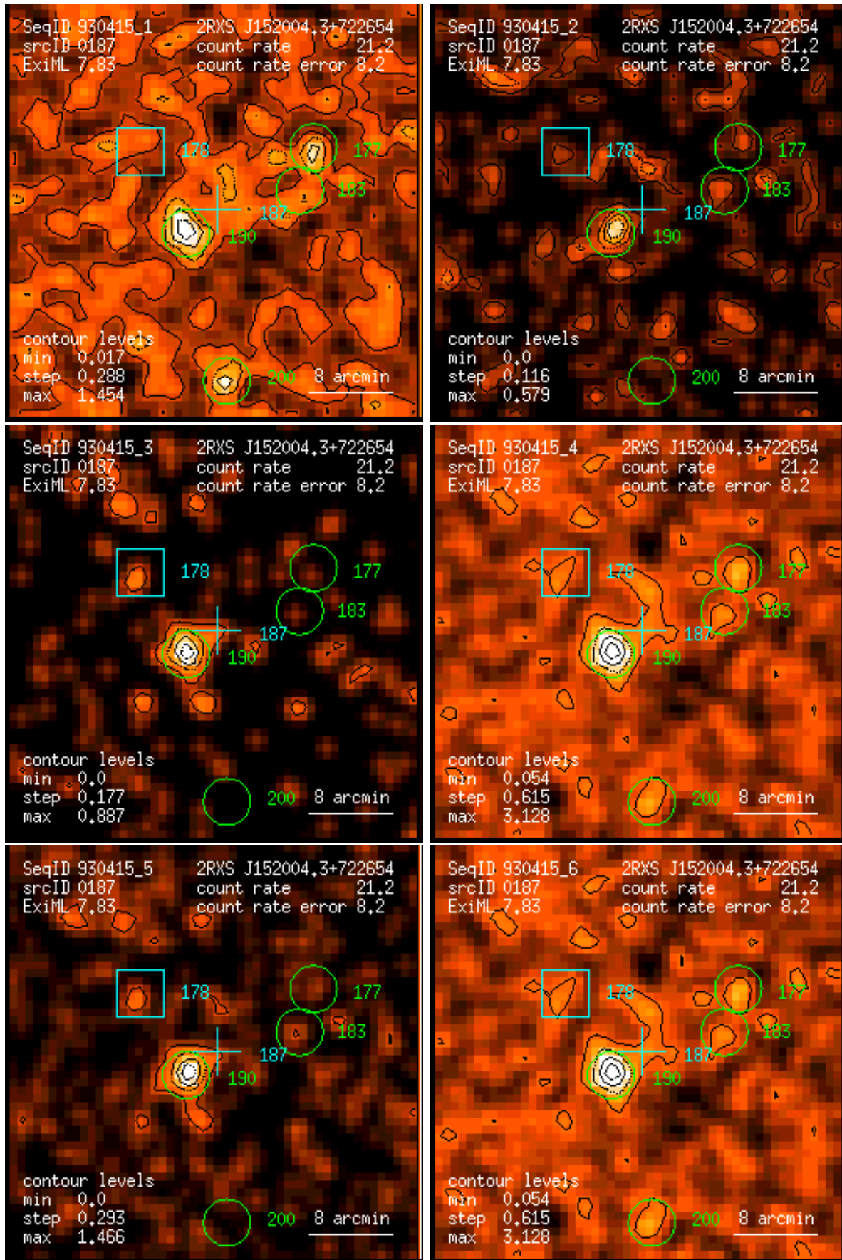
Figure 187: RASS 930415: detection 0187: band rate images, Gaussian filter: (1) PSPC channels 11 – 41, (2) 52 – 90, (3) 91 – 201, (4) 11 – 235, (5) 52 – 201, (6) 11 – 201. Broad band rates in counts/ks. Band rate contour levels in counts/ks/arcmin 2 .
