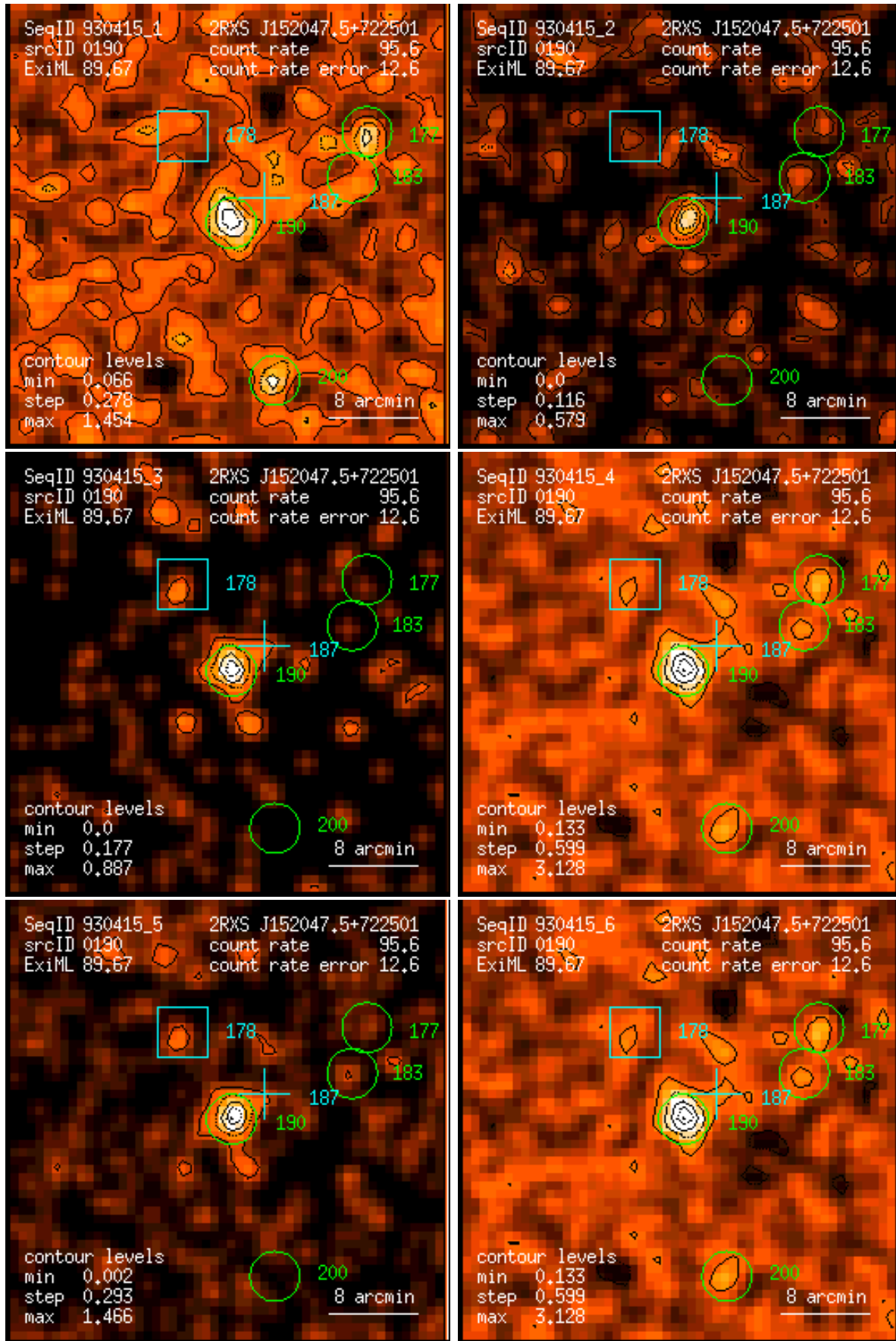
Figure 190: RASS 930415: detection 0190: band rate images, Gaussian filter: (1) PSPC channels 11 – 41, (2) 52 – 90, (3) 91 – 201, (4) 11 – 235, (5) 52 – 201, (6) 11 – 201. Broad band rates in counts/ks. Band rate contour levels in counts/ks/arcmin 2 .
