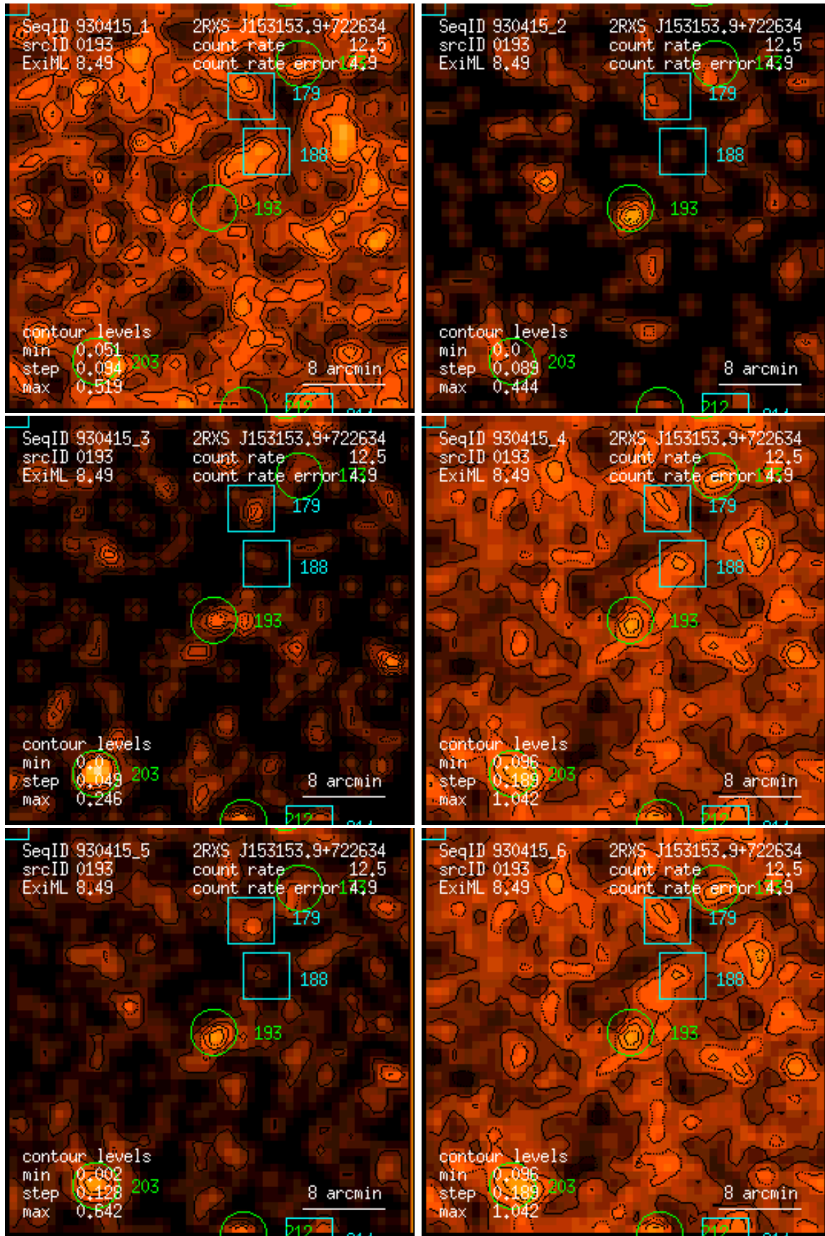
Figure 193: RASS 930415: detection 0193: band rate images, Gaussian filter: (1) PSPC channels 11 – 41, (2) 52 – 90, (3) 91 – 201, (4) 11 – 235, (5) 52 – 201, (6) 11 – 201. Broad band rates in counts/ks. Band rate contour levels in counts/ks/arcmin 2 .
