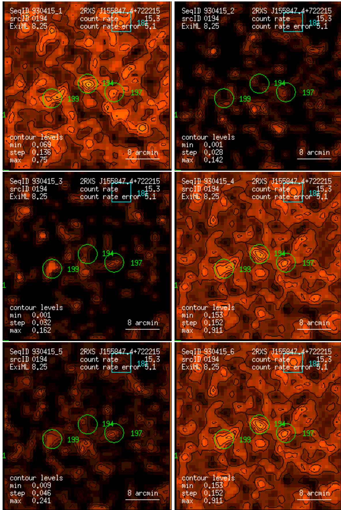
Figure 194: RASS 930415: detection 0194: band rate images, Gaussian filter: (1) PSPC channels 11 – 41, (2) 52 – 90, (3) 91 – 201, (4) 11 – 235, (5) 52 – 201, (6) 11 – 201. Broad band rates in counts/ks. Band rate contour levels in counts/ks/arcmin 2 .
