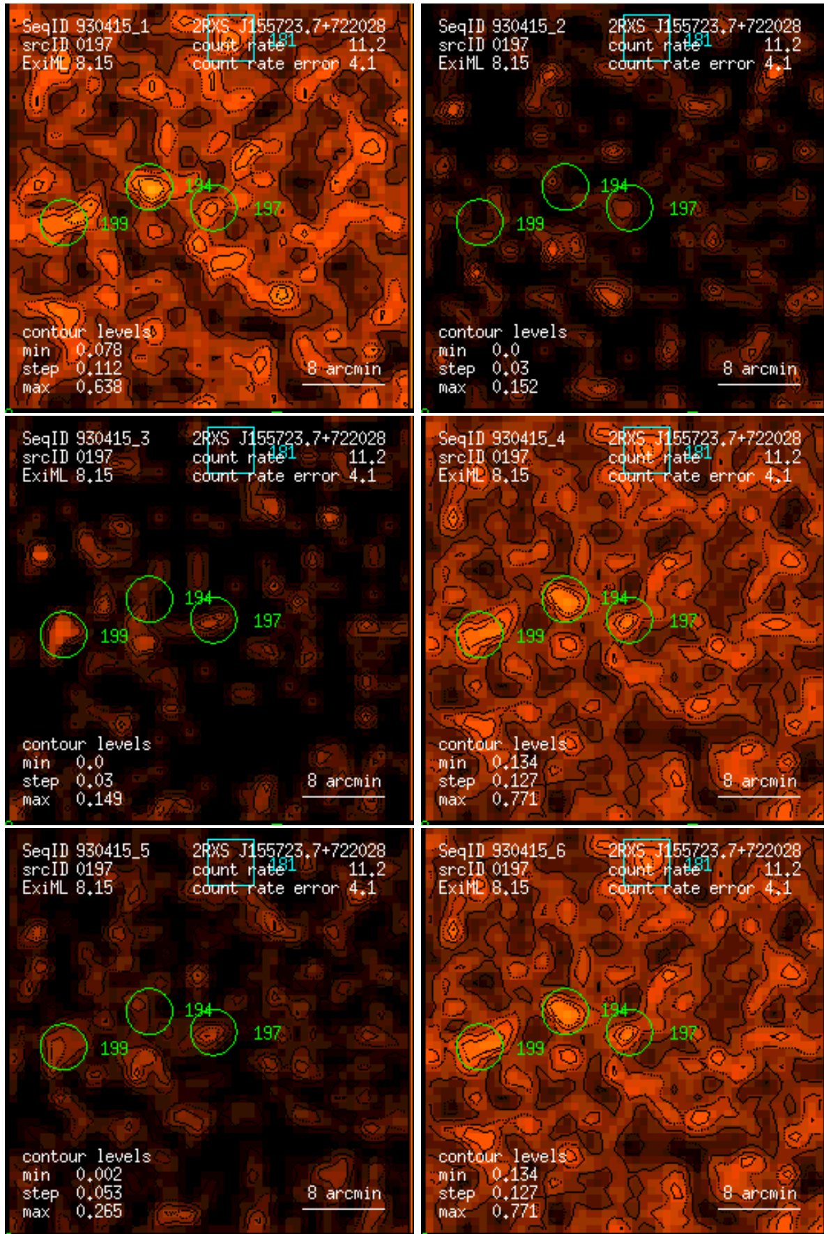
Figure 197: RASS 930415: detection 0197: band rate images, Gaussian filter: (1) PSPC channels 11 – 41, (2) 52 – 90, (3) 91 – 201, (4) 11 – 235, (5) 52 – 201, (6) 11 – 201. Broad band rates in counts/ks. Band rate contour levels in counts/ks/arcmin 2 .
