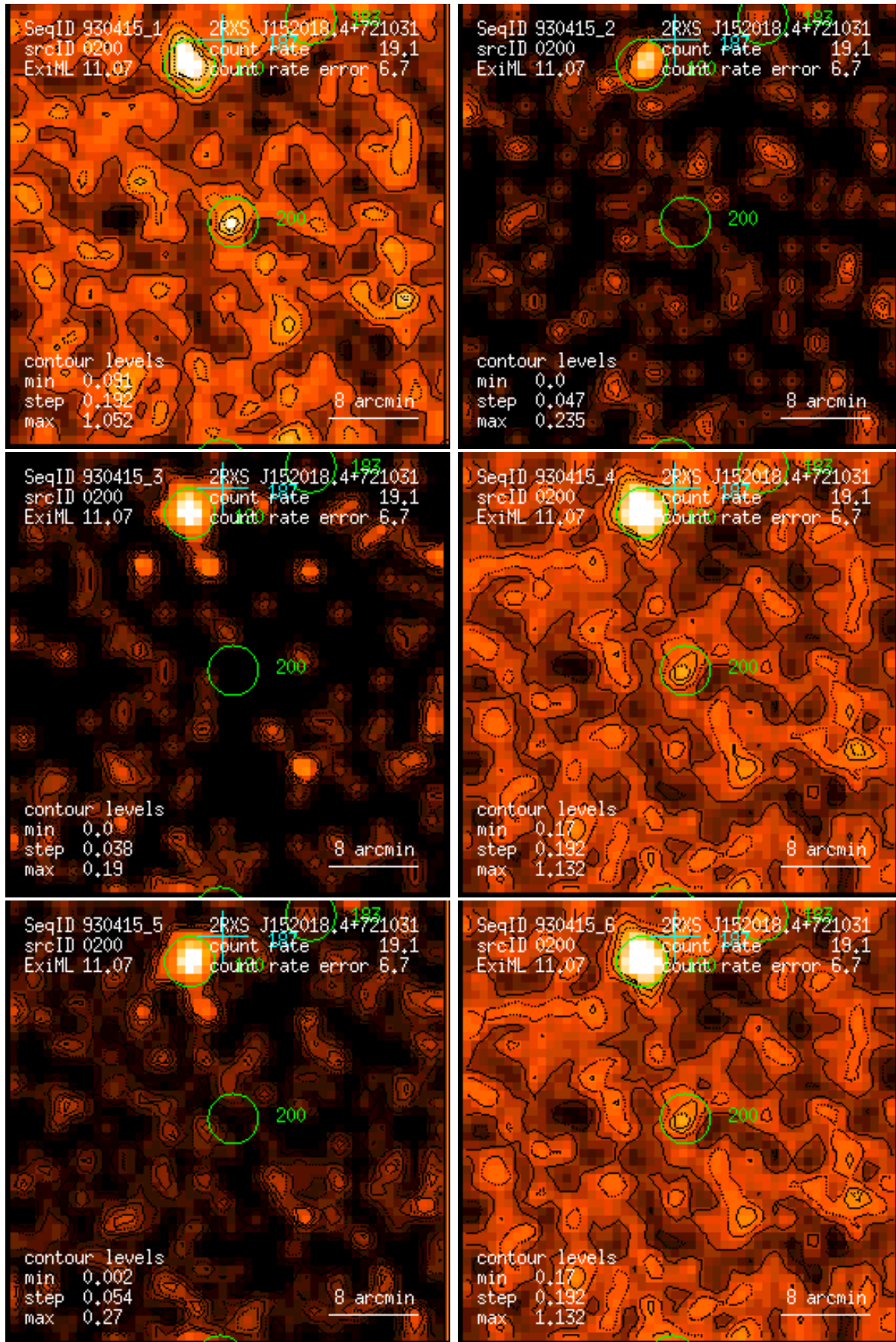
Figure 200: RASS 930415: detection 0200: band rate images, Gaussian filter: (1) PSPC channels 11 – 41, (2) 52 – 90, (3) 91 – 201, (4) 11 – 235, (5) 52 – 201, (6) 11 – 201. Broad band rates in counts/ks. Band rate contour levels in counts/ks/arcmin 2 .
