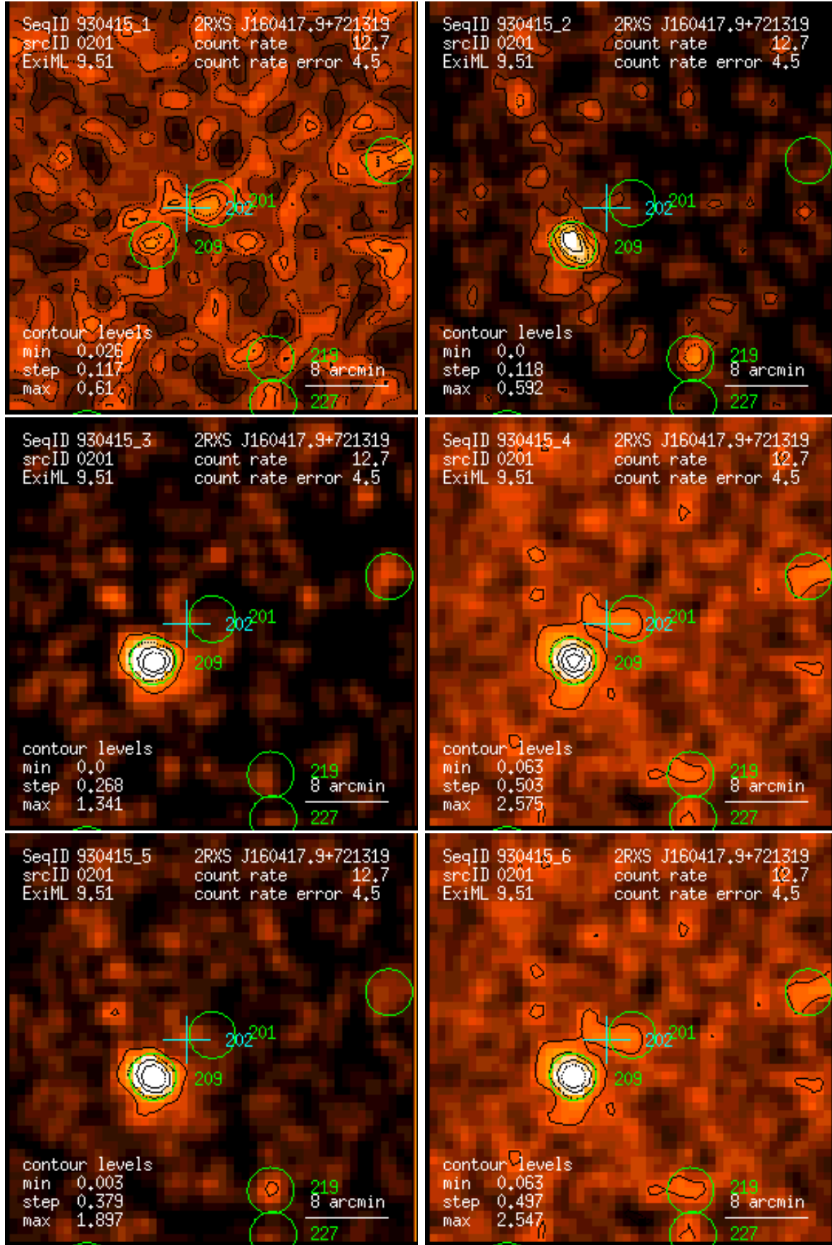
Figure 201: RASS 930415: detection 0201: band rate images, Gaussian filter: (1) PSPC channels 11 – 41, (2) 52 – 90, (3) 91 – 201, (4) 11 – 235, (5) 52 – 201, (6) 11 – 201. Broad band rates in counts/ks. Band rate contour levels in counts/ks/arcmin 2 .
