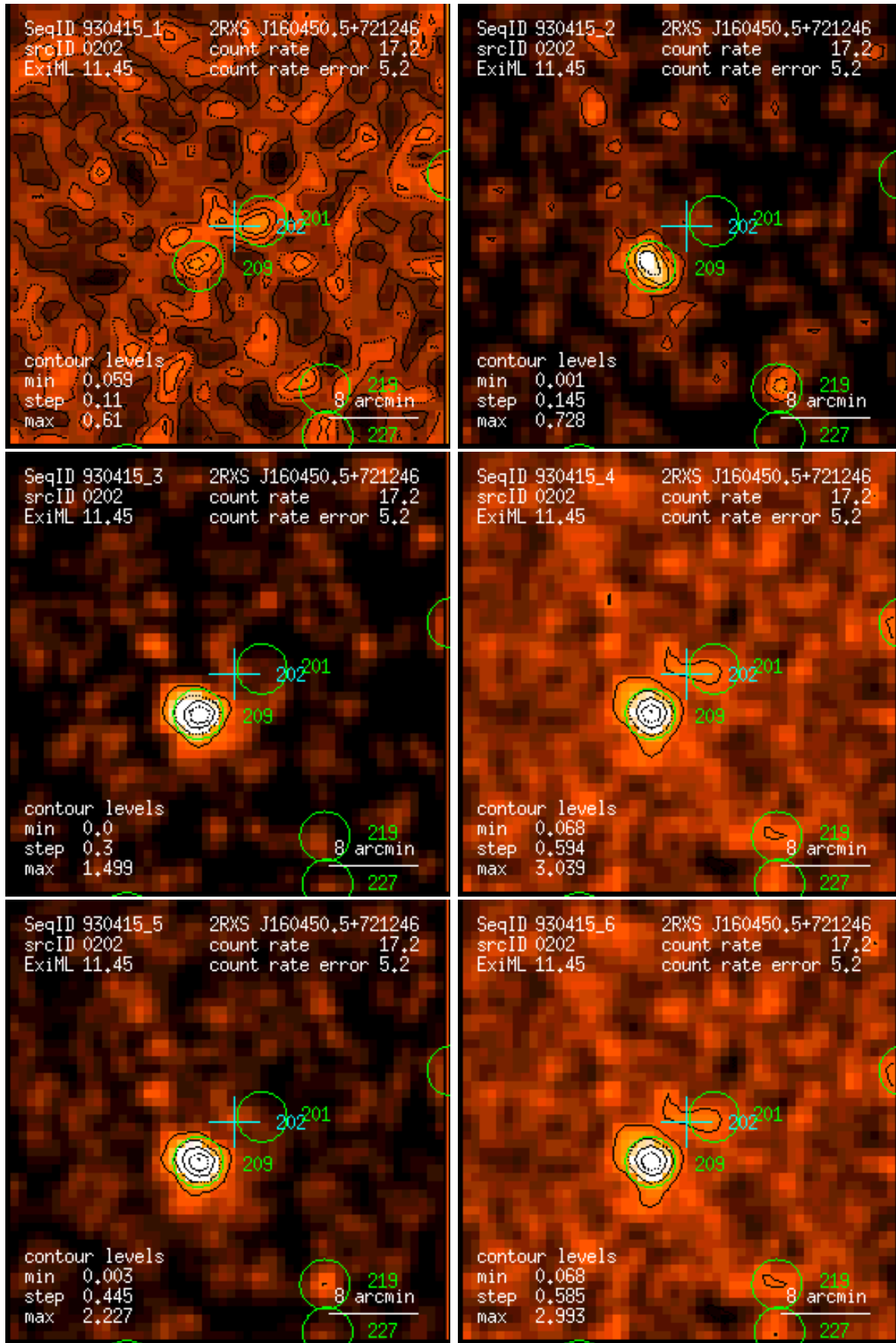
Figure 202: RASS 930415: detection 0202: band rate images, Gaussian filter: (1) PSPC channels 11 – 41, (2) 52 – 90, (3) 91 – 201, (4) 11 – 235, (5) 52 – 201, (6) 11 – 201. Broad band rates in counts/ks. Band rate contour levels in counts/ks/arcmin 2 .
