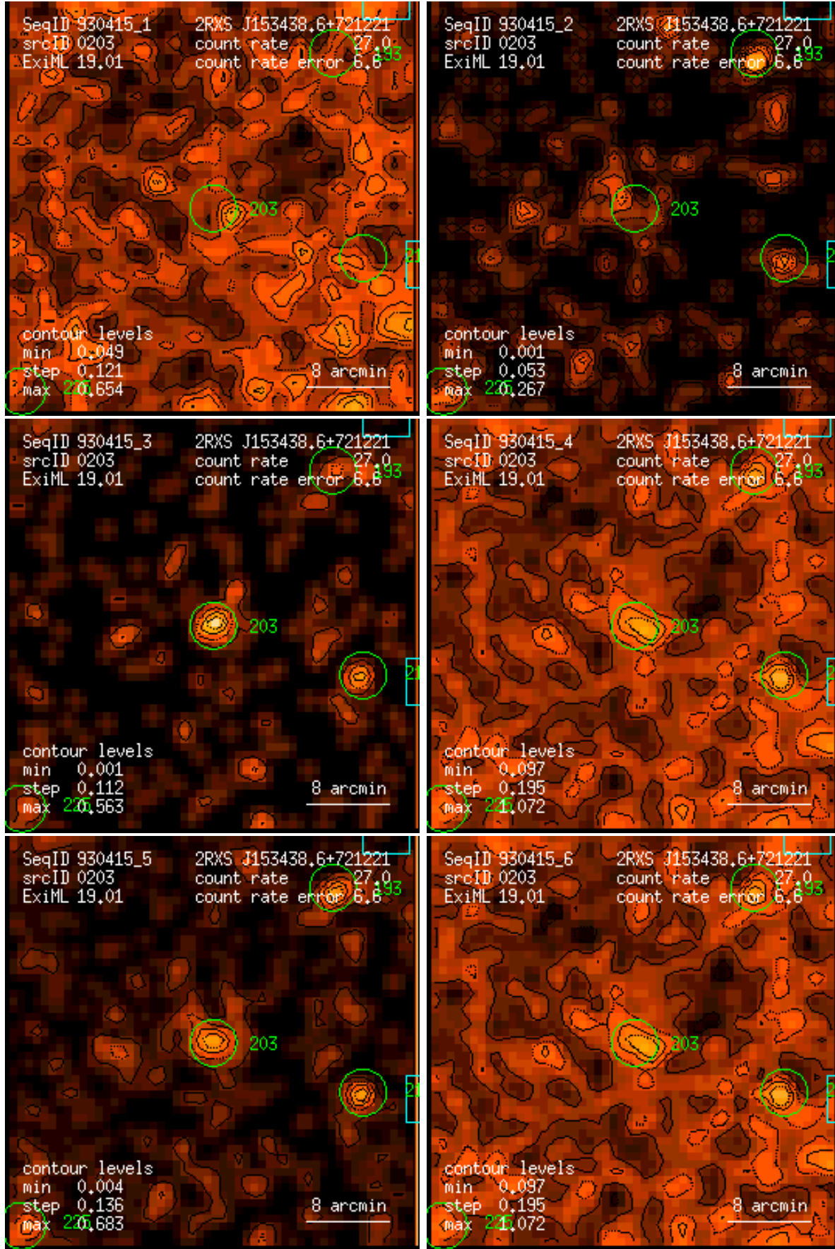
Figure 203: RASS 930415: detection 0203: band rate images, Gaussian filter: (1) PSPC channels 11 – 41, (2) 52 – 90, (3) 91 – 201, (4) 11 – 235, (5) 52 – 201, (6) 11 – 201. Broad band rates in counts/ks. Band rate contour levels in counts/ks/arcmin 2 .
