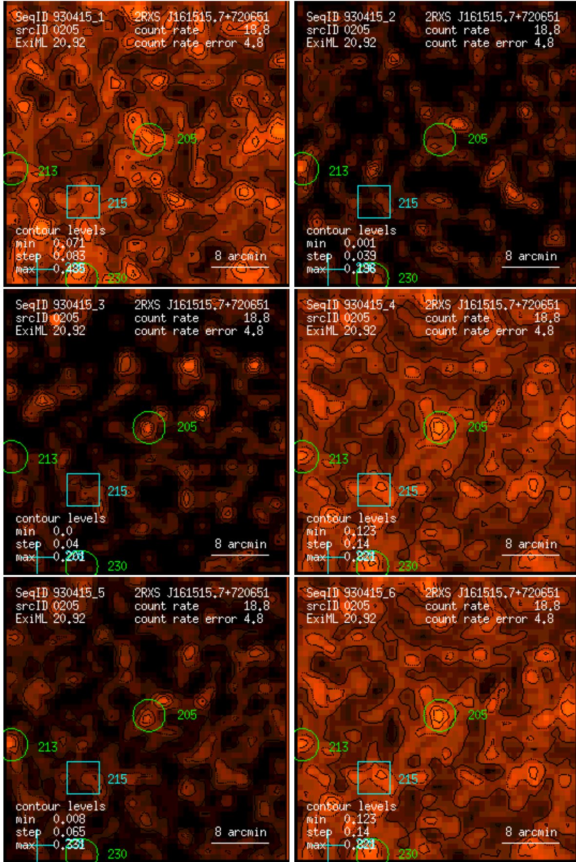
Figure 205: RASS 930415: detection 0205: band rate images, Gaussian filter: (1) PSPC channels 11 – 41, (2) 52 – 90, (3) 91 – 201, (4) 11 – 235, (5) 52 – 201, (6) 11 – 201. Broad band rates in counts/ks. Band rate contour levels in counts/ks/arcmin 2 .
