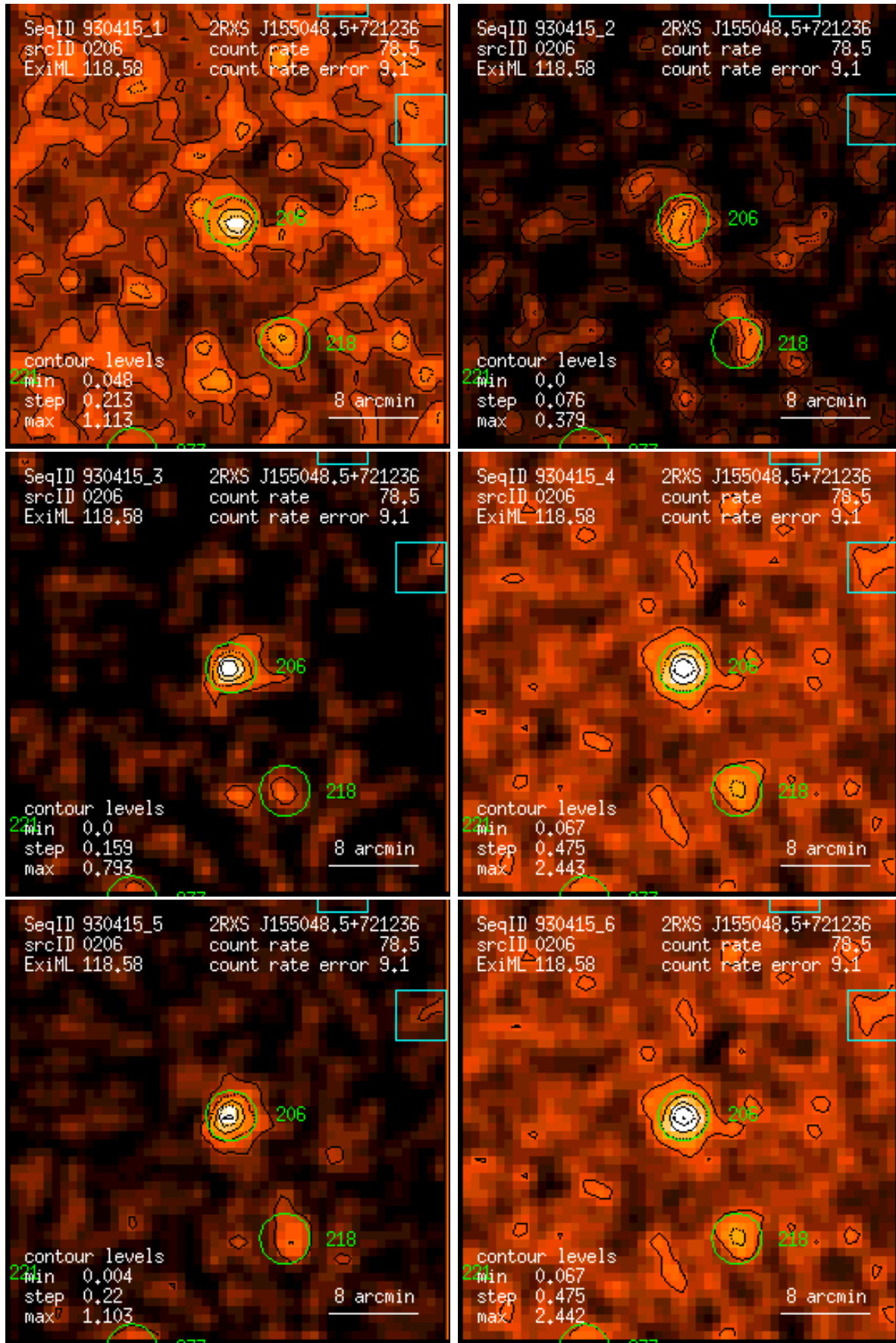
Figure 206: RASS 930415: detection 0206: band rate images, Gaussian filter: (1) PSPC channels 11 – 41, (2) 52 – 90, (3) 91 – 201, (4) 11 – 235, (5) 52 – 201, (6) 11 – 201. Broad band rates in counts/ks. Band rate contour levels in counts/ks/arcmin 2 .
