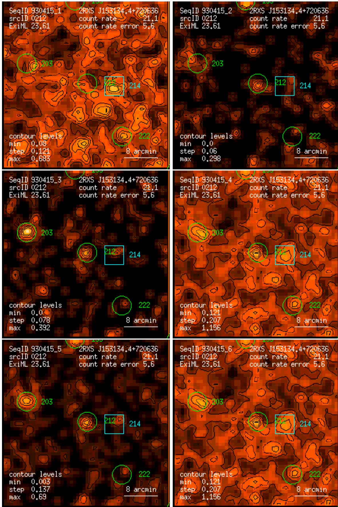
Figure 212: RASS 930415: detection 0212: band rate images, Gaussian filter: (1) PSPC channels 11 – 41, (2) 52 – 90, (3) 91 – 201, (4) 11 – 235, (5) 52 – 201, (6) 11 – 201. Broad band rates in counts/ks. Band rate contour levels in counts/ks/arcmin 2 .
