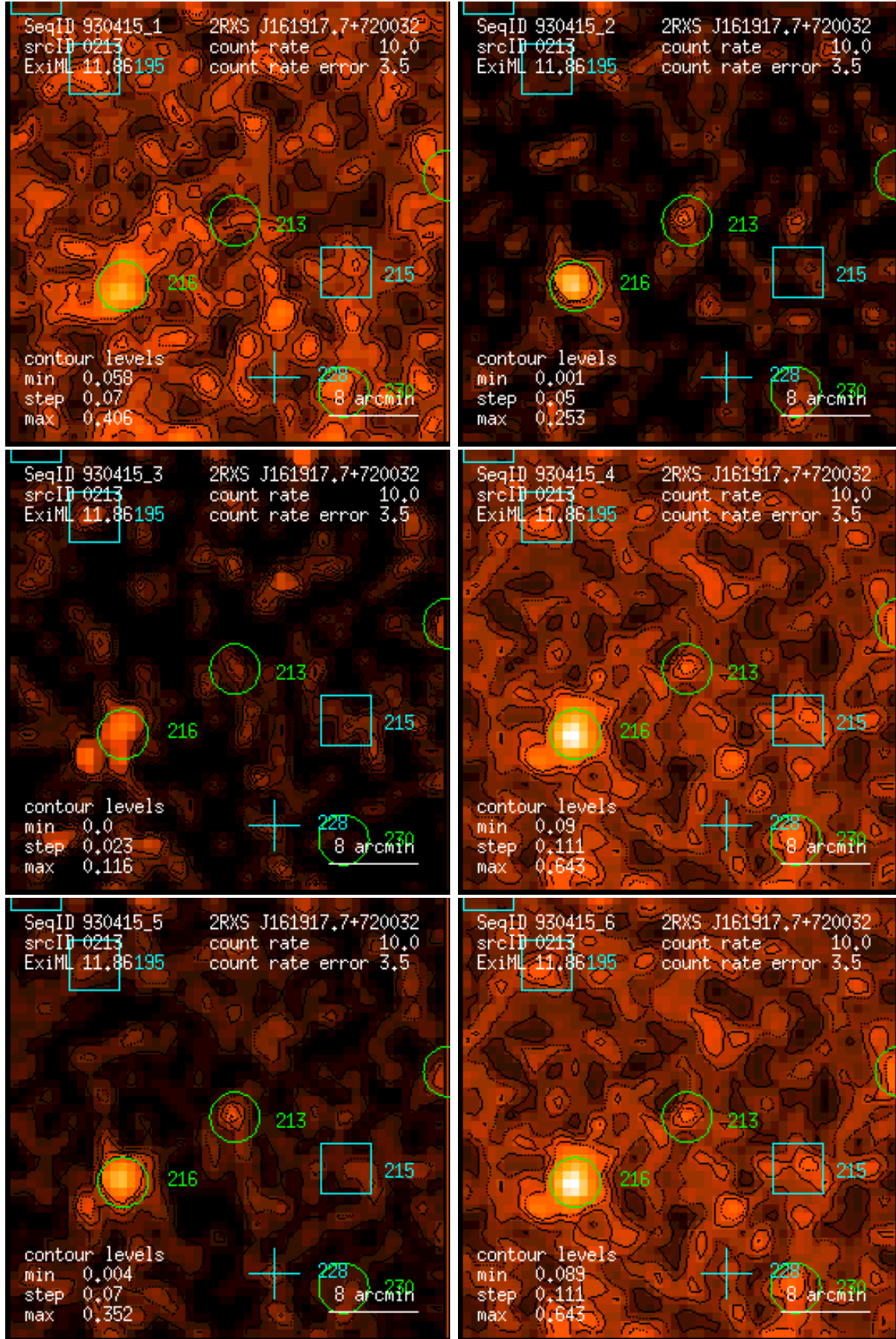
Figure 213: RASS 930415: detection 0213: band rate images, Gaussian filter: (1) PSPC channels 11 – 41, (2) 52 – 90, (3) 91 – 201, (4) 11 – 235, (5) 52 – 201, (6) 11 – 201. Broad band rates in counts/ks. Band rate contour levels in counts/ks/arcmin 2 .
