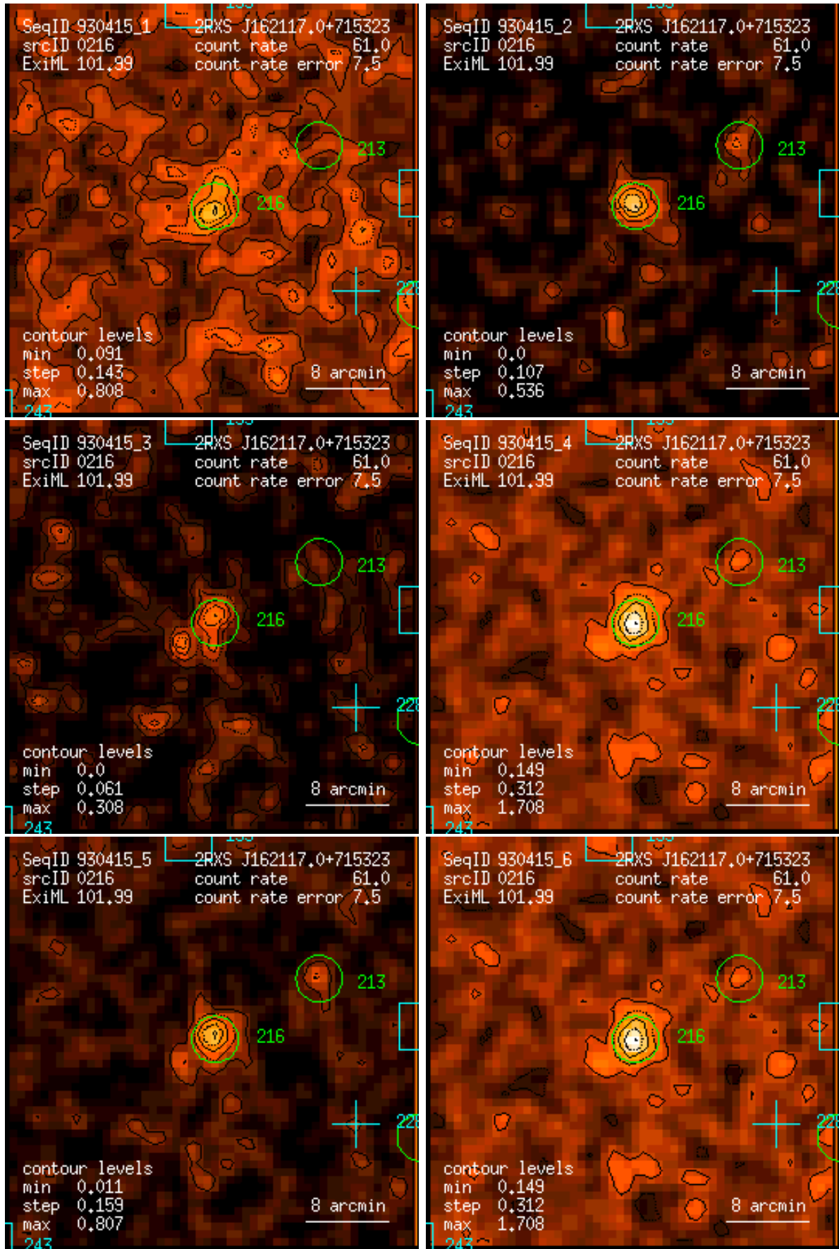
Figure 216: RASS 930415: detection 0216: band rate images, Gaussian filter: (1) PSPC channels 11 – 41, (2) 52 – 90, (3) 91 – 201, (4) 11 – 235, (5) 52 – 201, (6) 11 – 201. Broad band rates in counts/ks. Band rate contour levels in counts/ks/arcmin 2 .
