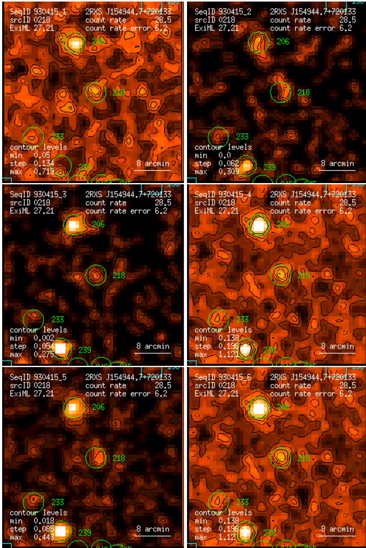
Figure 218: RASS 930415: detection 0218: band rate images, Gaussian filter: (1) PSPC channels 11 – 41, (2) 52 – 90, (3) 91 – 201, (4) 11 – 235, (5) 52 – 201, (6) 11 – 201. Broad band rates in counts/ks. Band rate contour levels in counts/ks/arcmin 2 .
