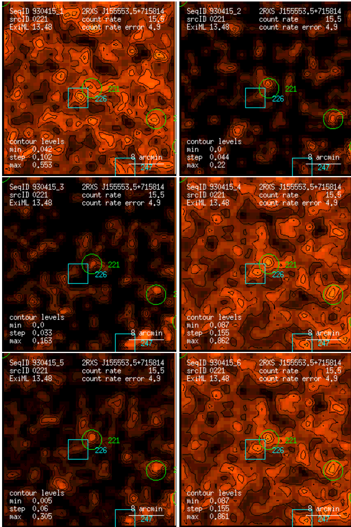
Figure 221: RASS 930415: detection 0221: band rate images, Gaussian filter: (1) PSPC channels 11 – 41, (2) 52 – 90, (3) 91 – 201, (4) 11 – 235, (5) 52 – 201, (6) 11 – 201. Broad band rates in counts/ks. Band rate contour levels in counts/ks/arcmin 2 .
