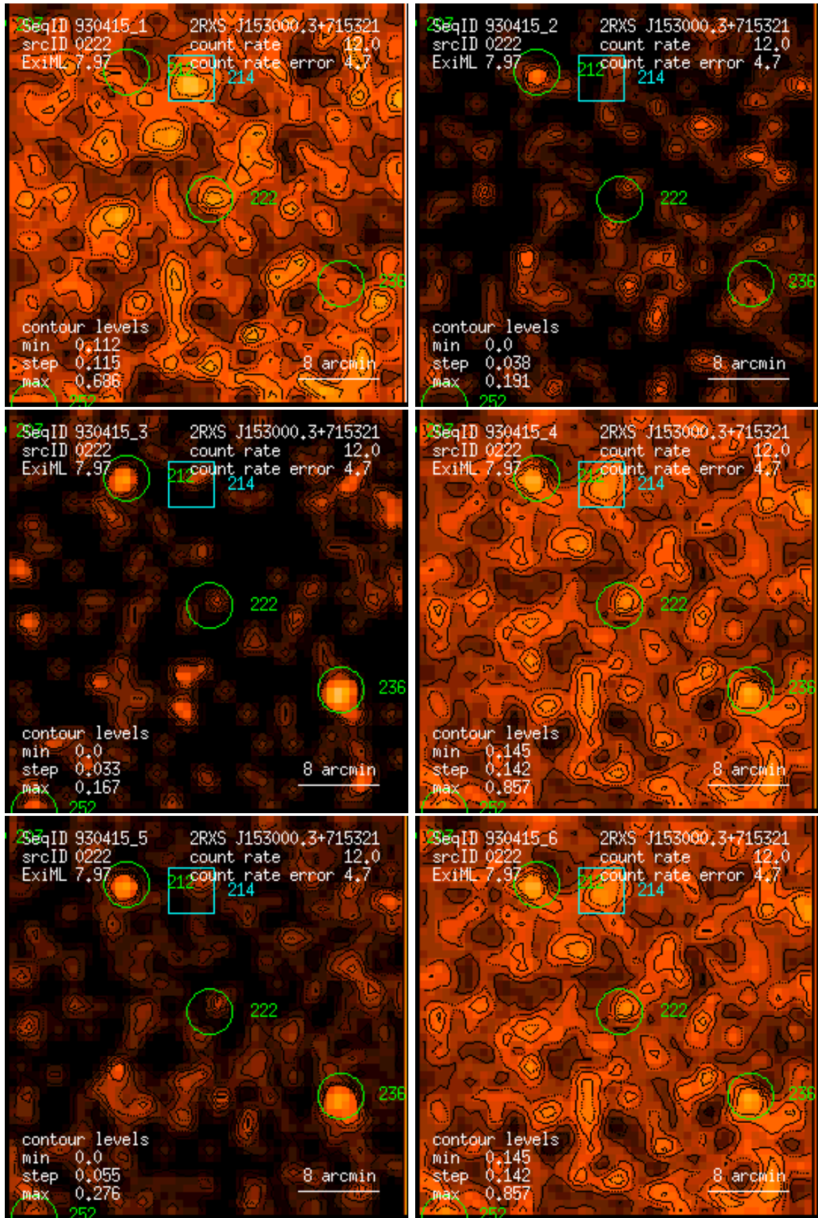
Figure 222: RASS 930415: detection 0222: band rate images, Gaussian filter: (1) PSPC channels 11 – 41, (2) 52 – 90, (3) 91 – 201, (4) 11 – 235, (5) 52 – 201, (6) 11 – 201. Broad band rates in counts/ks. Band rate contour levels in counts/ks/arcmin 2 .
